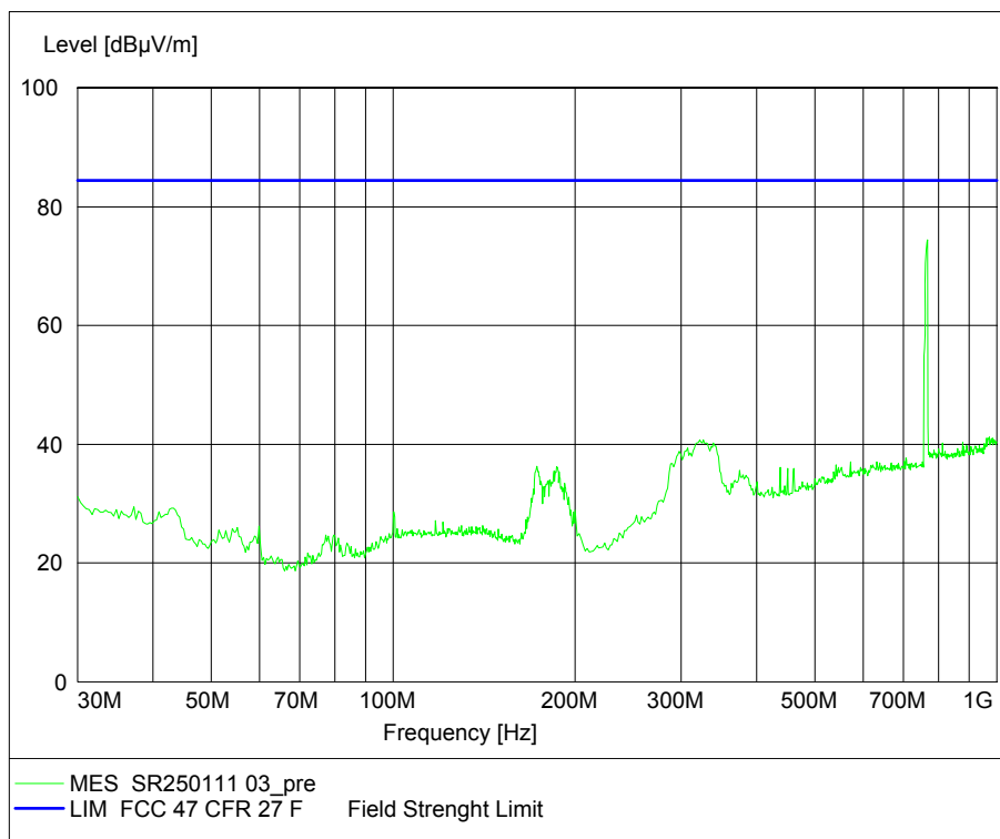
Figure 7-266: Radiated Emission (30MHz – 1GHz) (5MHz Channel BW)
