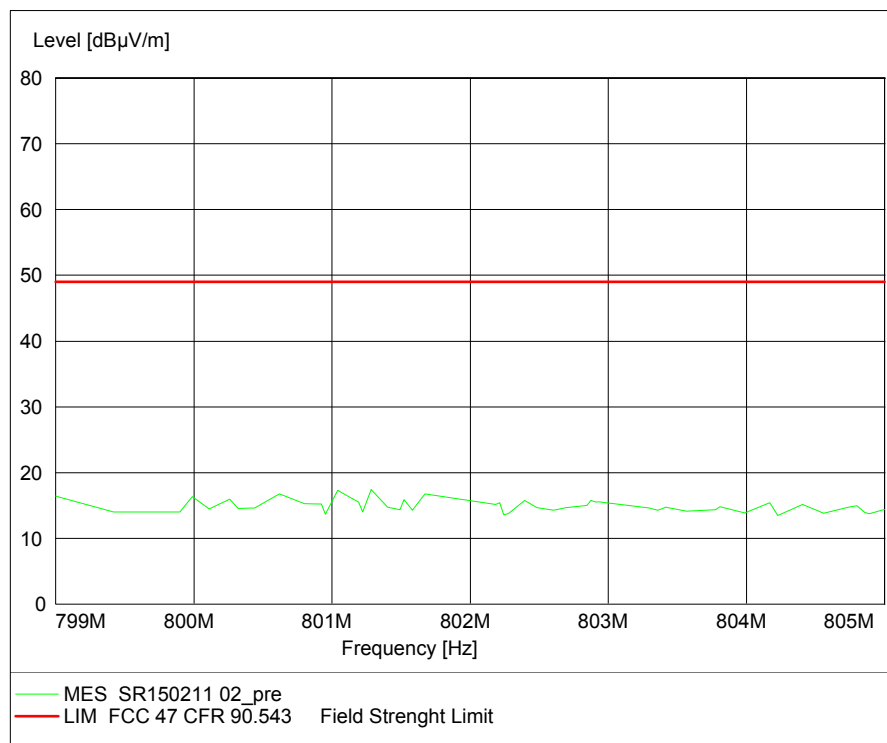
Figure 7-270: Radiated Emission (799MHz – 805MHz) (5MHz Channel BW)
