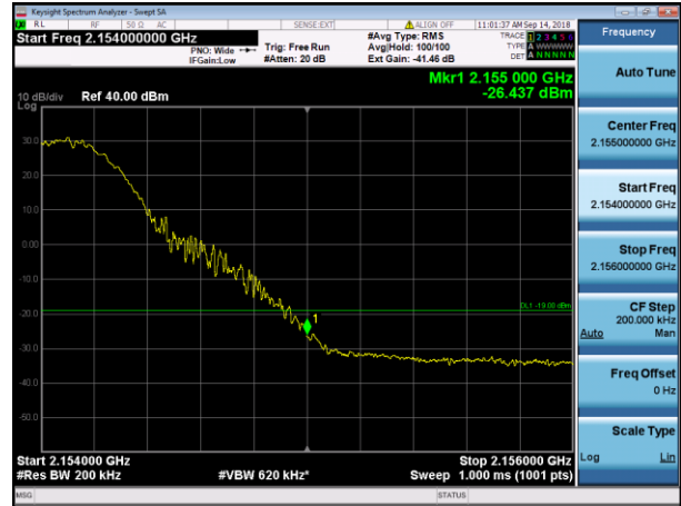
LTE20_Top Channel_UBE_2154 to 2156MHz
