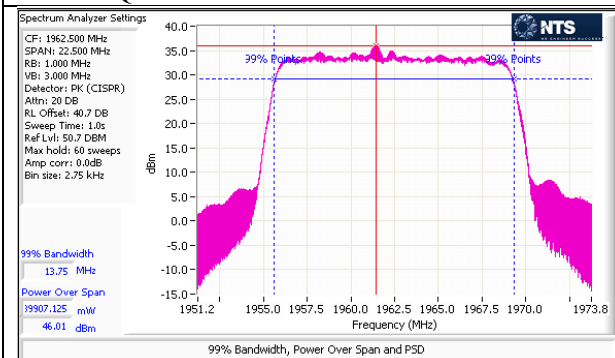
Port D – 16QAM – 15M – Center Channel – Peak
