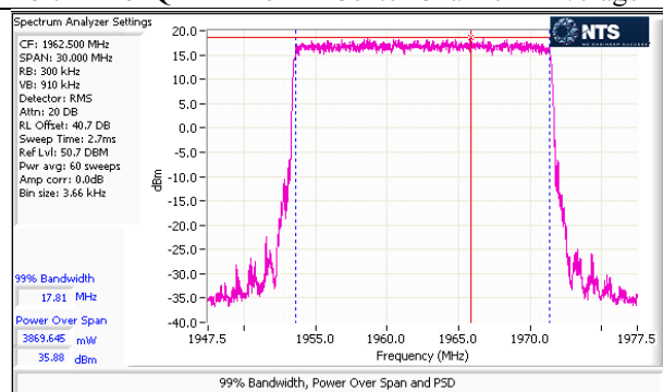
Port M – 64QAM – 20M – Center Channel – Average
