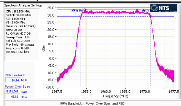
Port M – 16QAM – 20M – Center Channel – Peak
