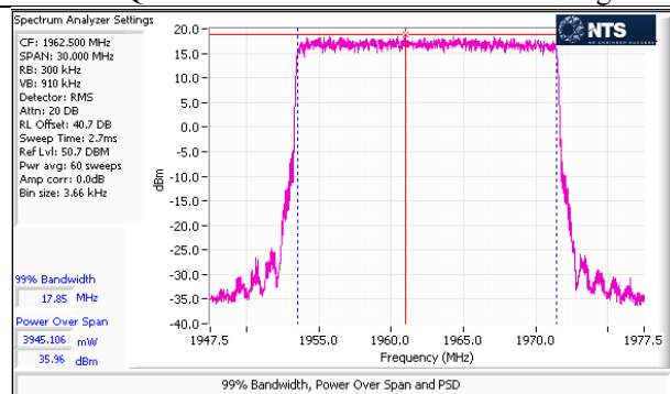
Port M – 16QAM – 20M – Center Channel – Average
