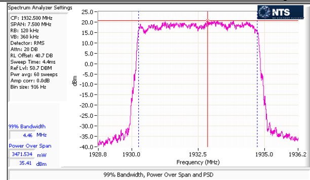
Port D – 64QAM – 5M – Bottom Channel – Average
