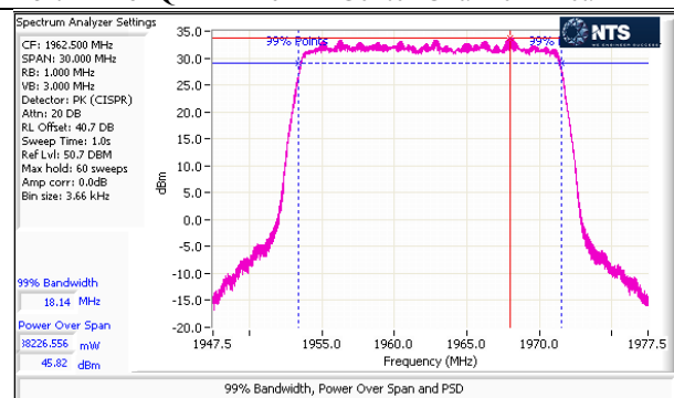
Port M – 64QAM – 20M – Center Channel – Peak
