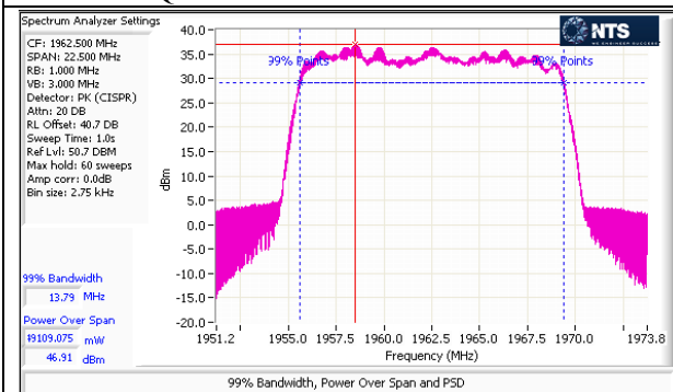
Port D – 64QAM – 15M – Center Channel – Peak
