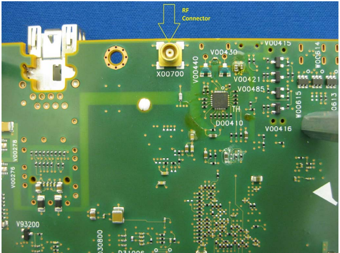
Close Up of BT RF Port
