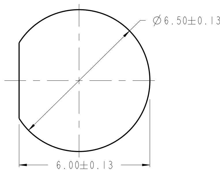
PANEL CUTOUT DETAILS SCALE 10:1
