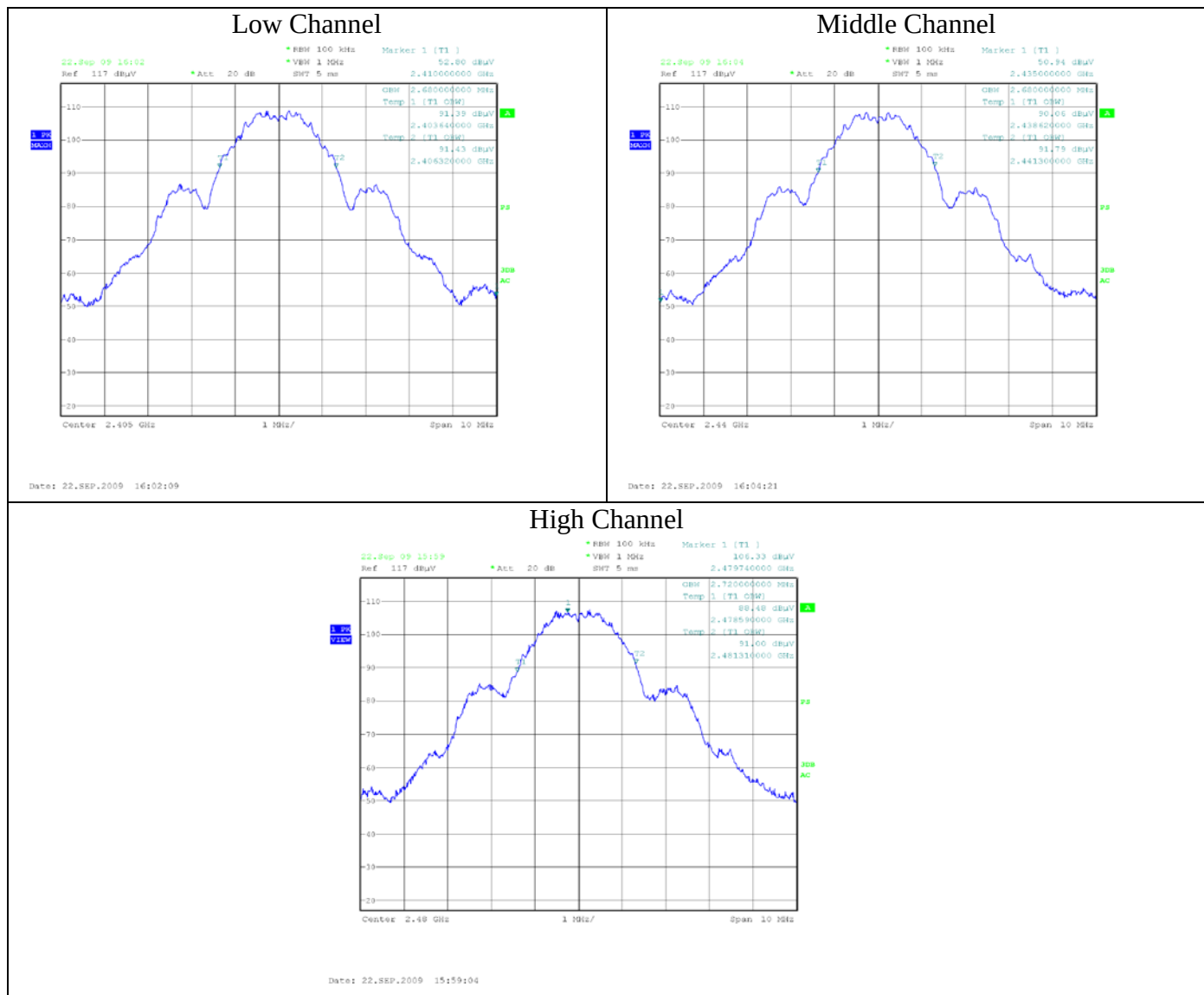
Figure 30 99% Power Bandwidth Graphs
