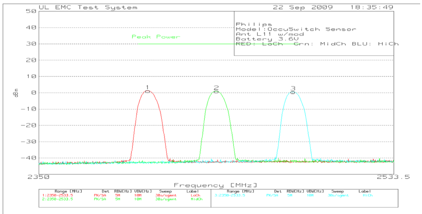
Figure 29 Maximum Peak Output Power Graph, L11
