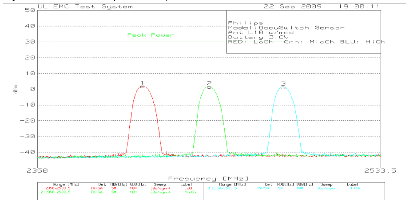
Figure 28 Maximum Peak Output Power Graph, L10
