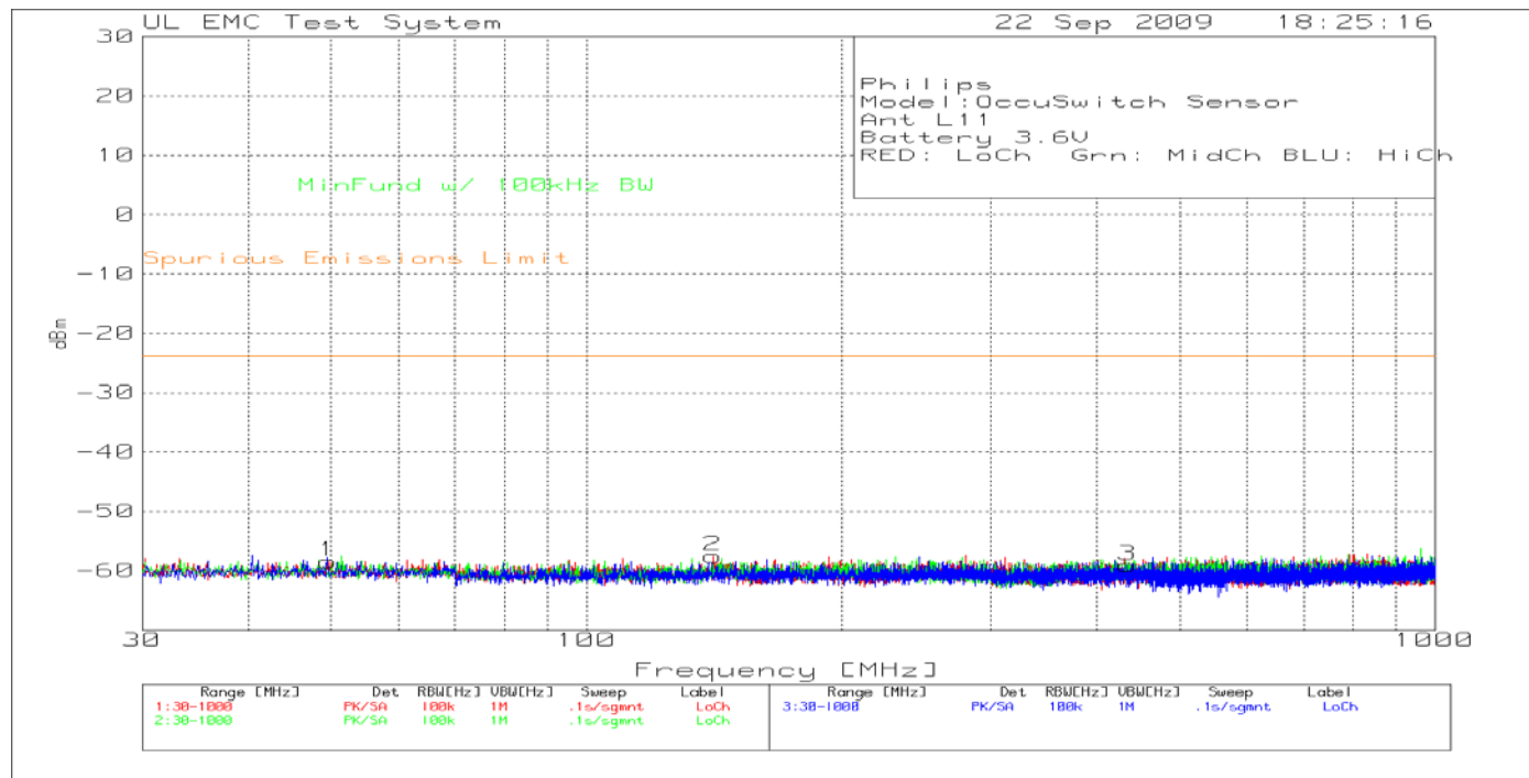
Figure 6 30MHz-1GHz Antenna (L11) Port Spurious Emissions Plots TX Mode, Low, Middle and High Channels.
