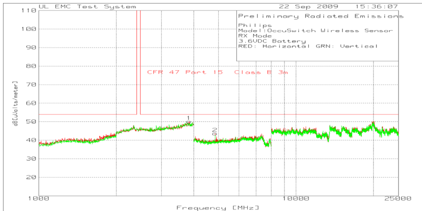
Figure 3 Radiated Emissions Graph 1GHz – 25GHz
