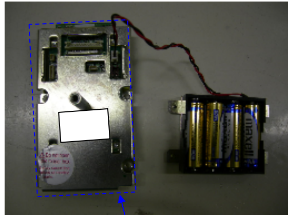
Metal case
