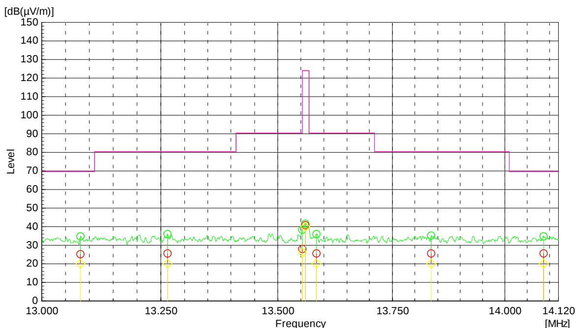
Figure 7: Field Strength of Fundamental, Spectral Diagram, Mode B
