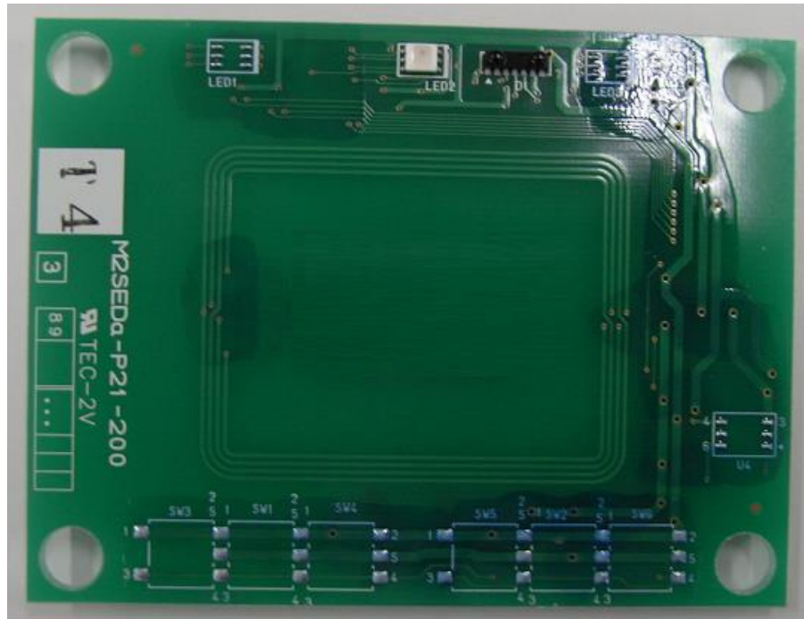
TOP View
