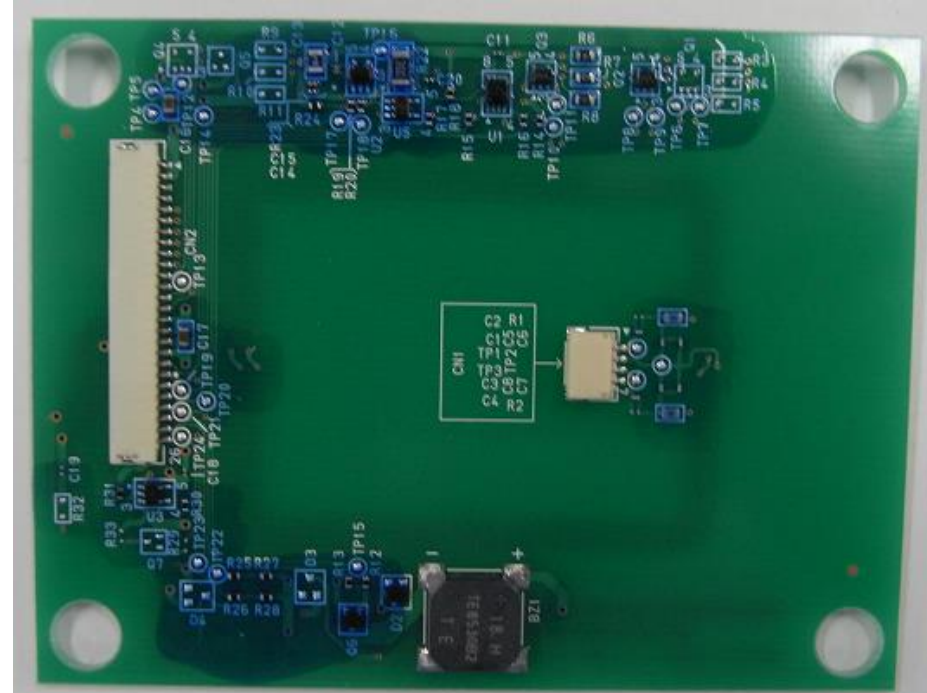
Bottom View
