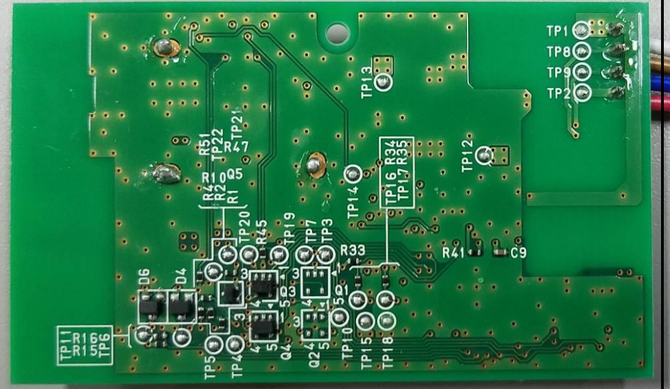
Bottom View
