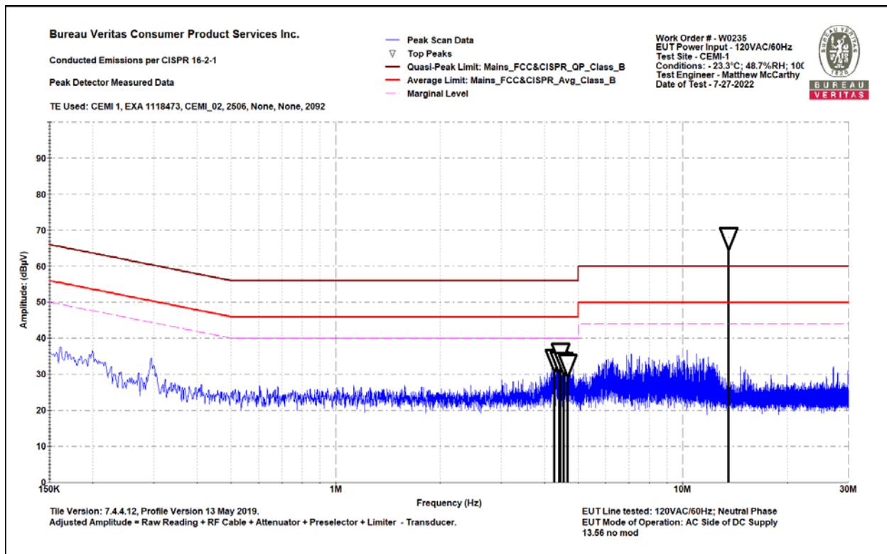
0.15 – 30MHz Neutral Peak (with production antenna)
