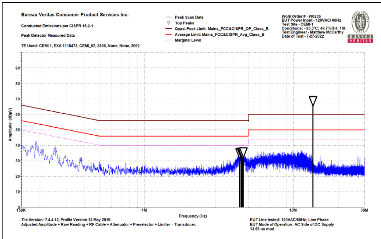
0.15 - 30MHz Line Peak (with production antenna)
