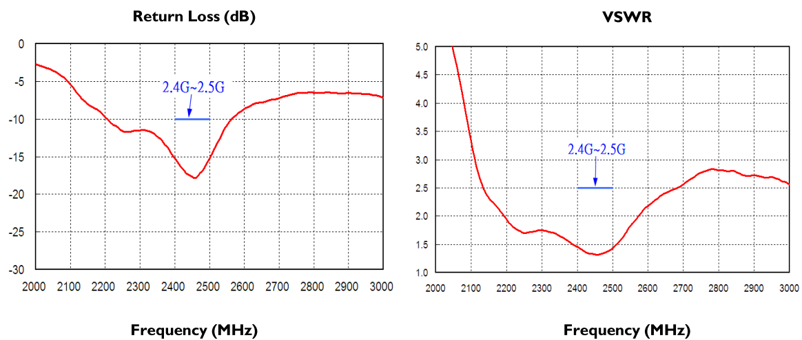
Fig. 3 Return loss & VSWR Measurement
