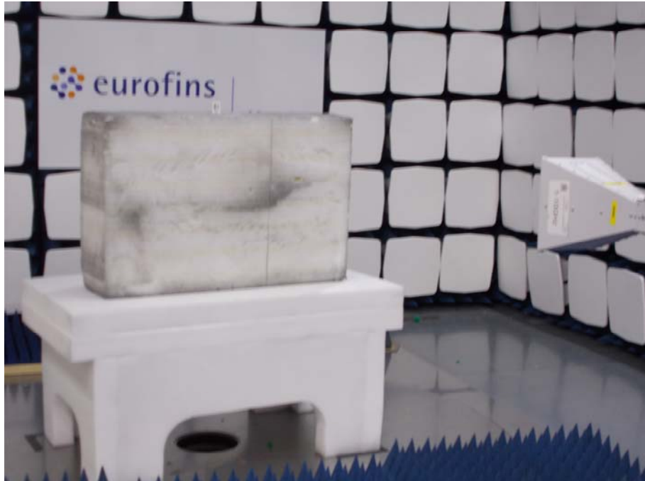
Radiated emissions, Pre-scan, > 1000 MHz
