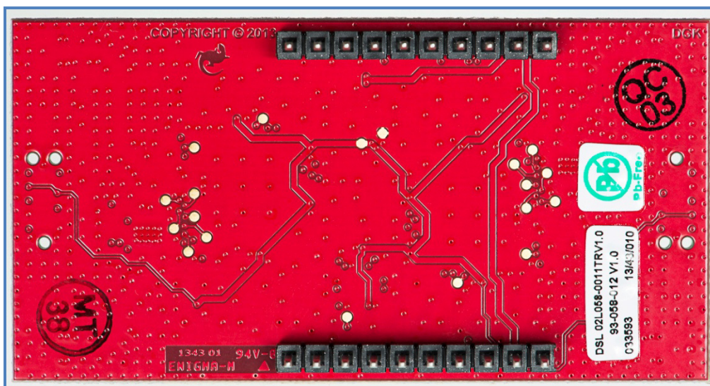
FIGURE 2 - BOTTOM SIDE OF PCB
