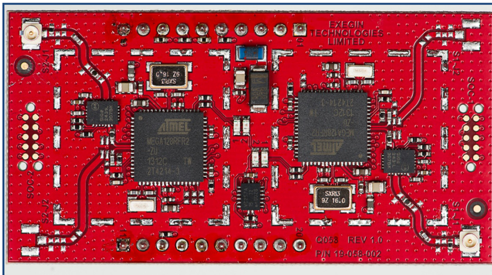
FIGURE 1 - EUT, SHIELDS REMOVED
