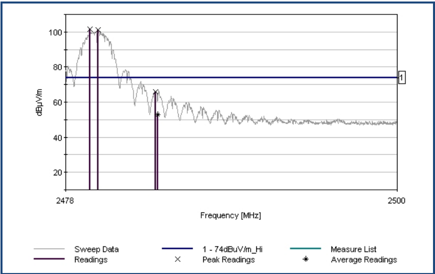
FIGURE 16 - UPPER BAND EDGE – HI CHANNEL
