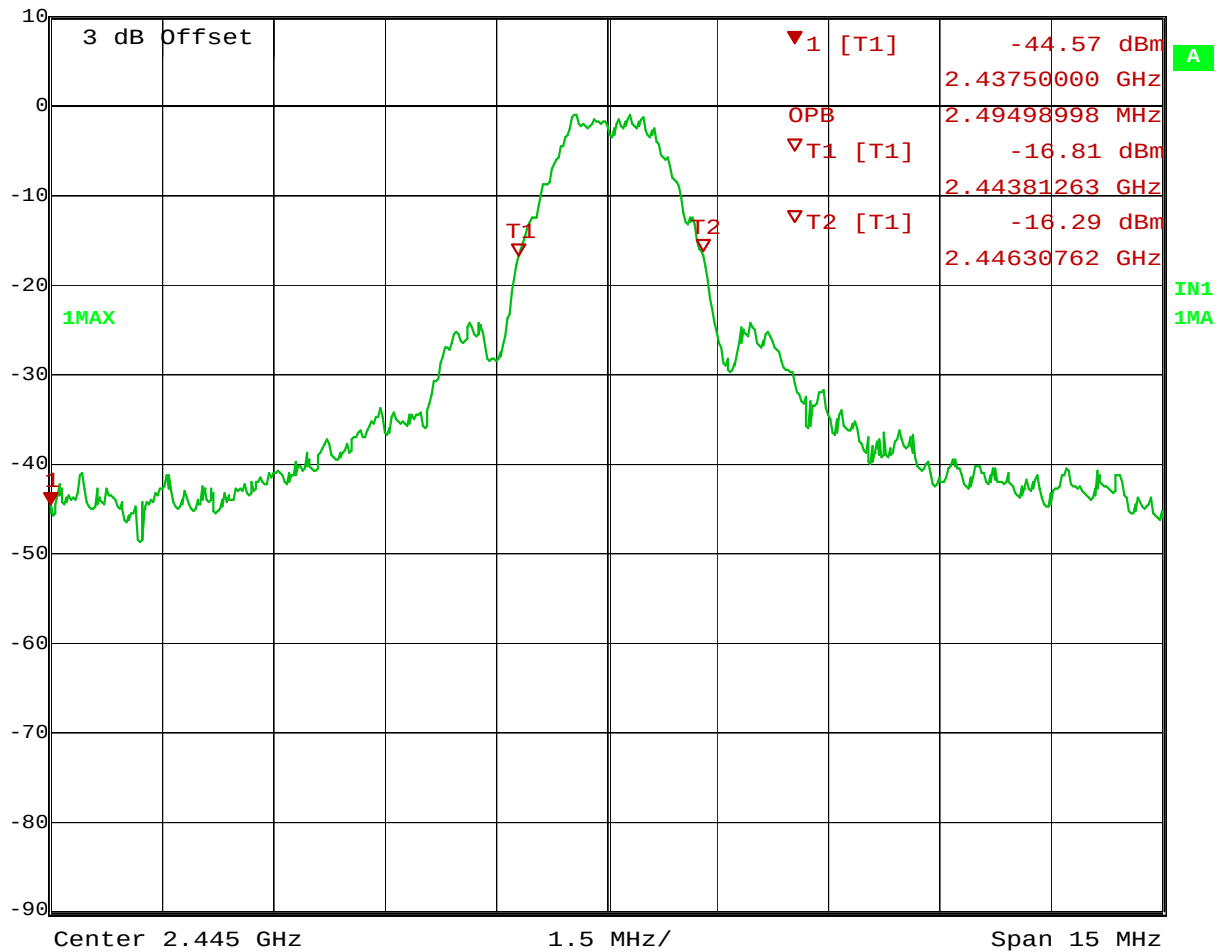
99% Power Bandwidth Plot (Channel 18)
