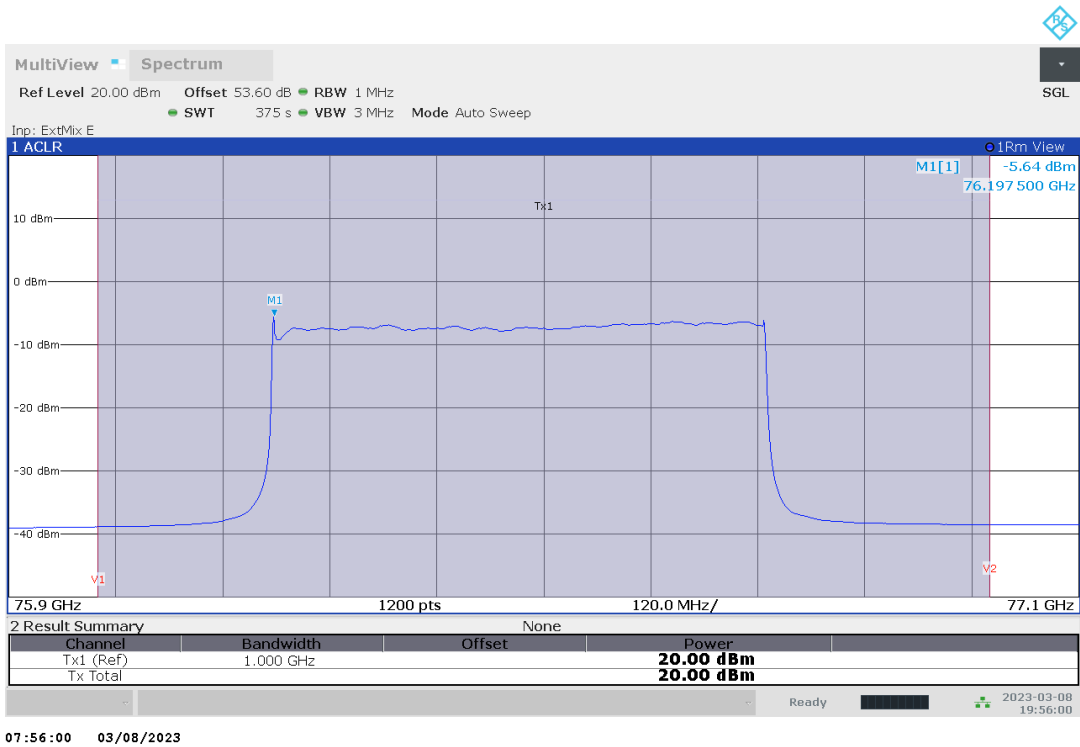
Plot no. 3: Mean Power EIRP, RMS detector / Channel Power, DUT 3 beam 2, T nom , V nom
