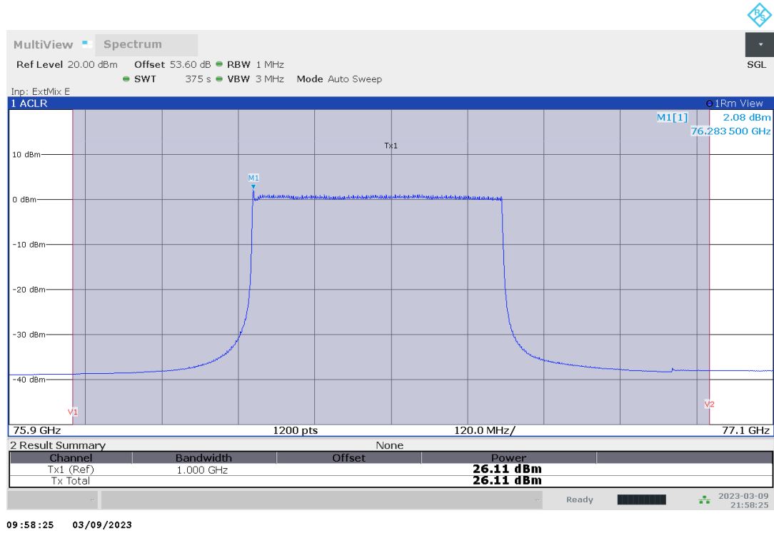
Plot no. 1: Mean Power EIRP, RMS detector / Channel Power, DUT 1 normal mode, T_{nom} , V_{nom}
