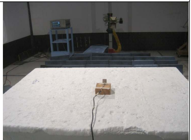
Radiated Emissions (1-18GHz) – Rear View
