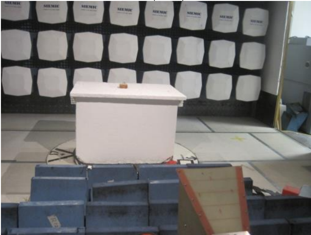
Radiated Emissions (1-18GHz) – Front View
