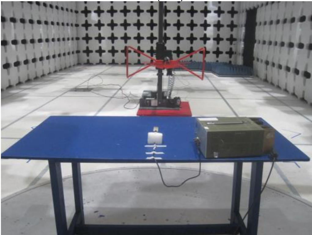
Radiated Emissions (<1GHz) – Rear View
