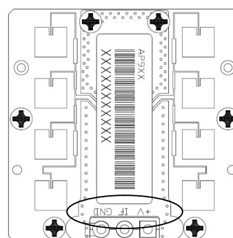
Figure 3: Terminals designation
