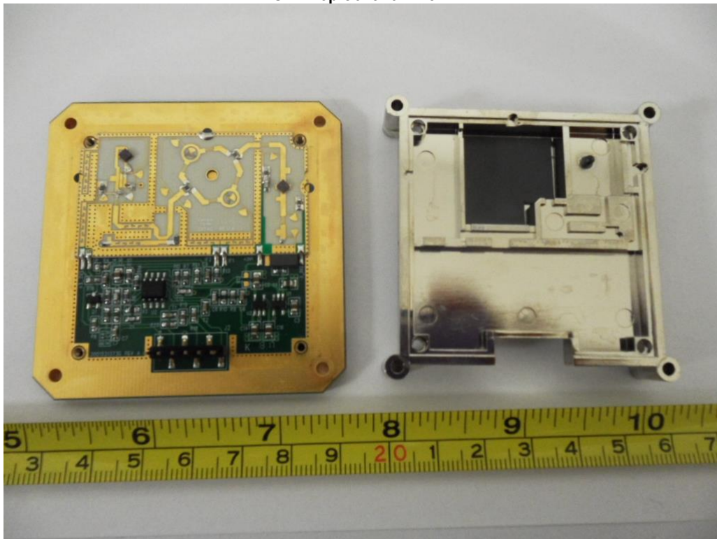
EUT – Top Cover off View 1
