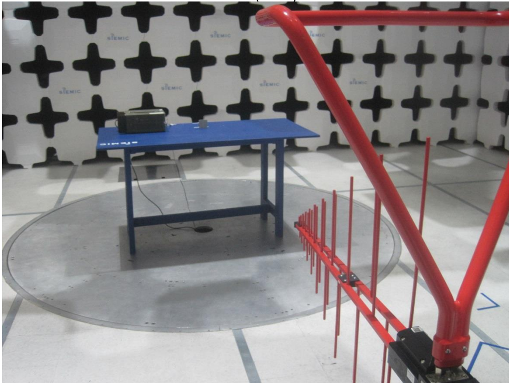
Radiated Emissions (<1GHz) – Front View
