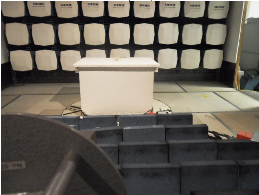
Radiated Emissions (>18GHz) – Front View
