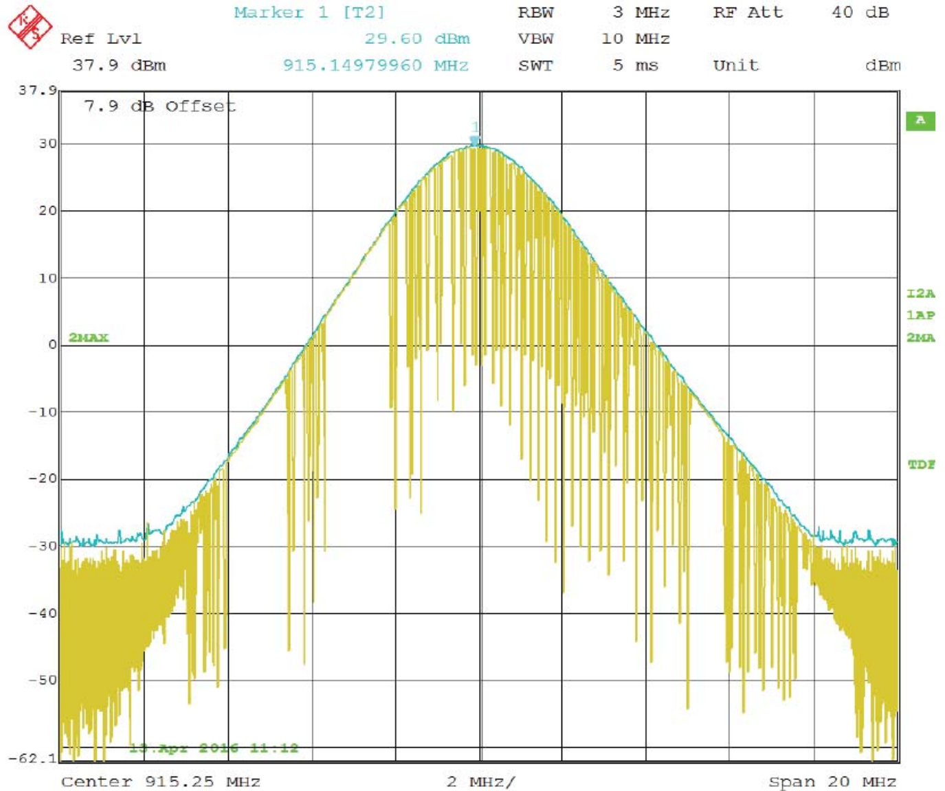
Peak Power Output – Middle Channel – Configuration #1 – Port #4 Worst Case
