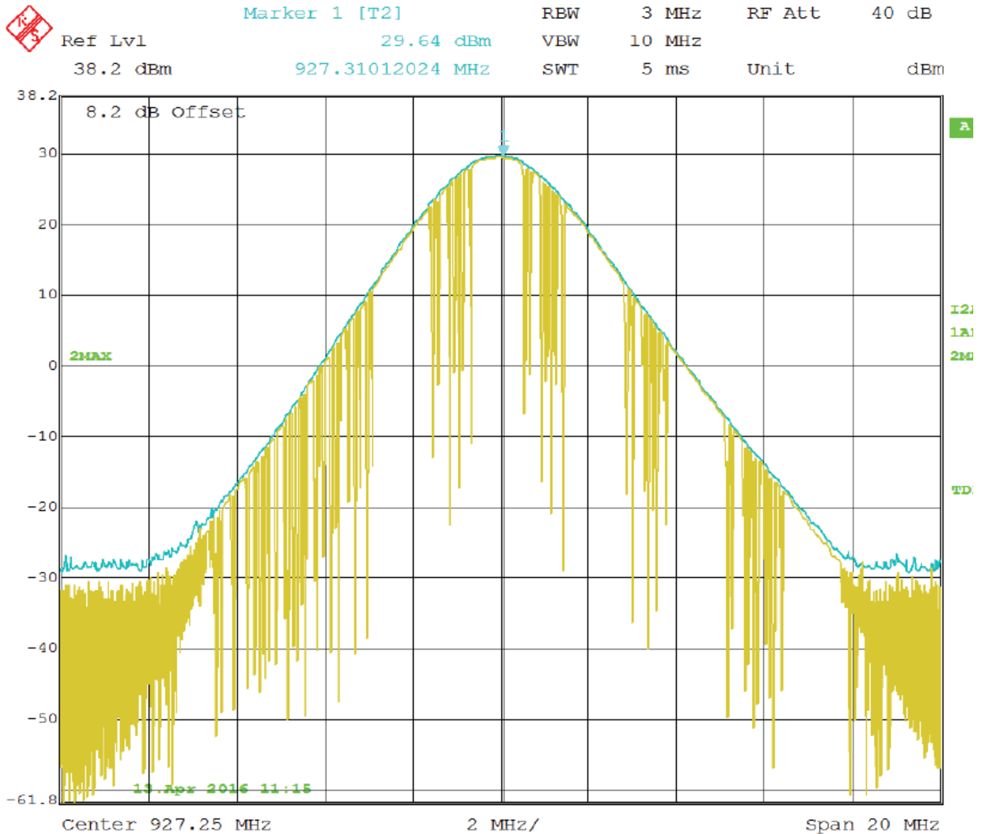
Peak Power Output – High Channel – Configuration #1 – Port #4 Worst Case
