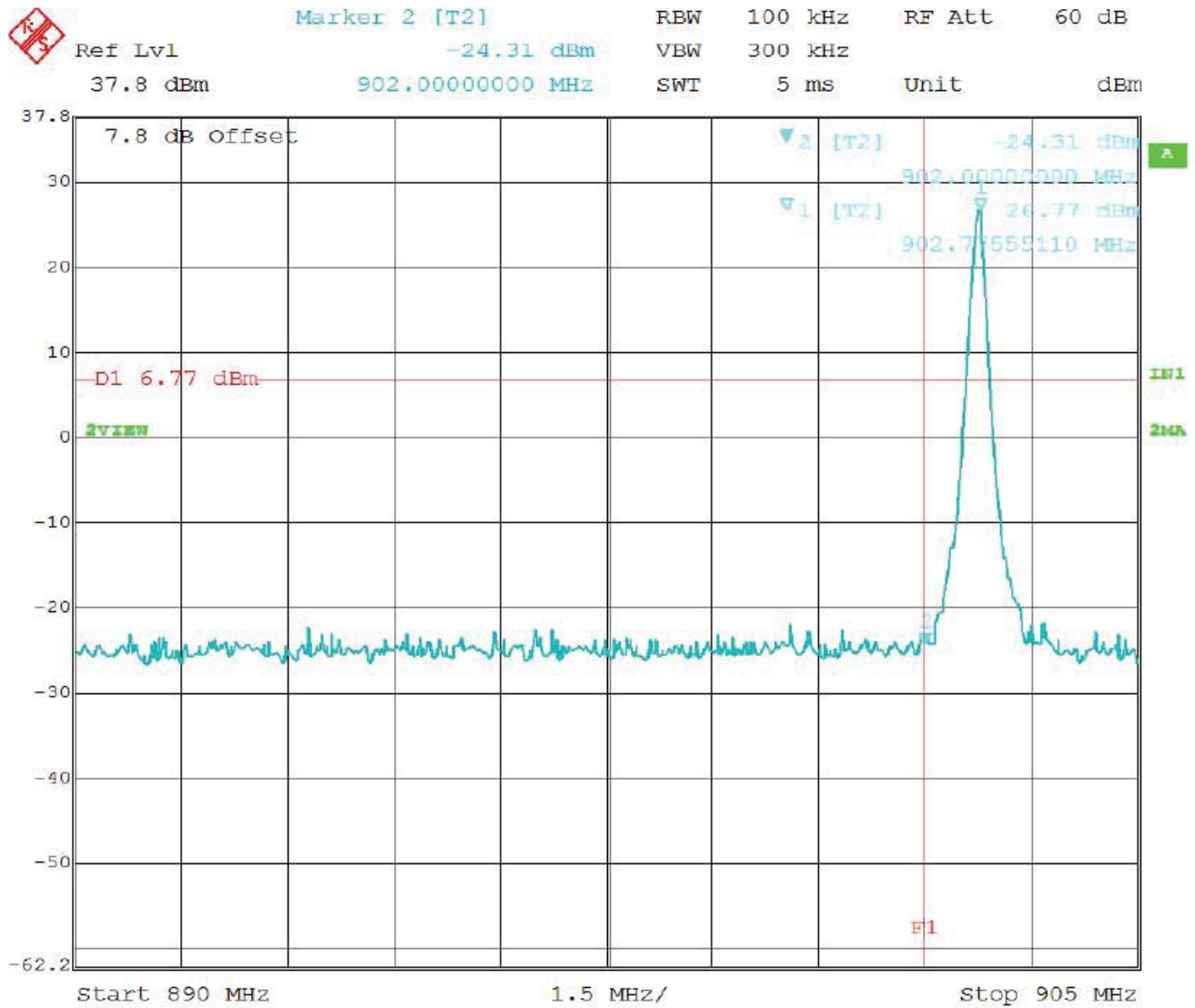
Band Edge – Low Channel – Fixed Frequency Mode – Configuration #2 – Port #1 Worst Case
