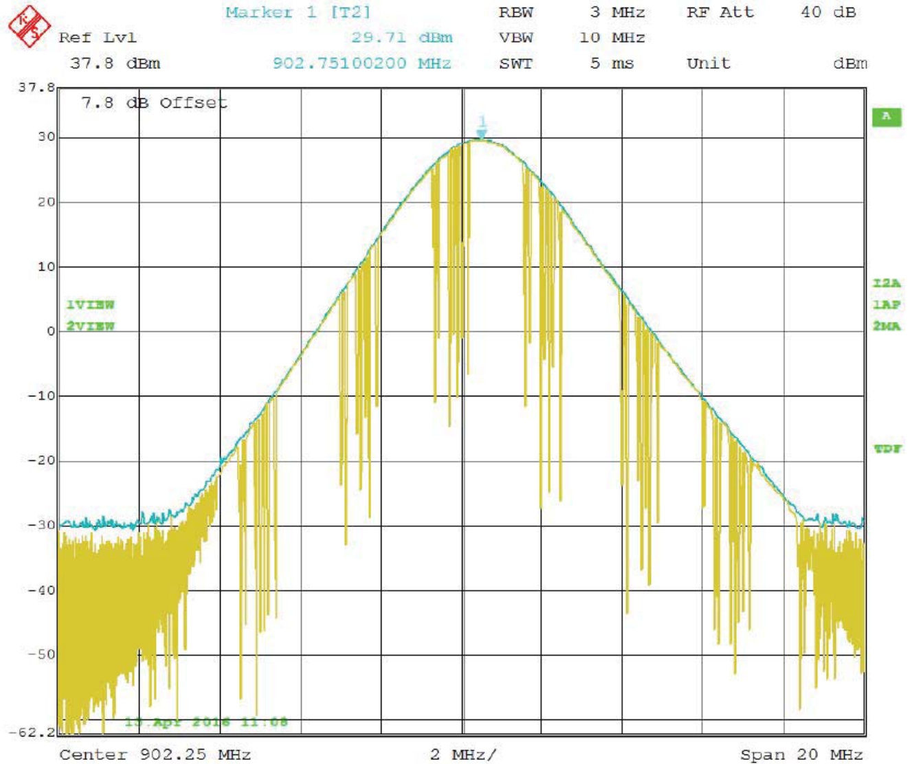
Peak Power Output – Low Channel – Configuration #1 – Port #4 Worst Case
