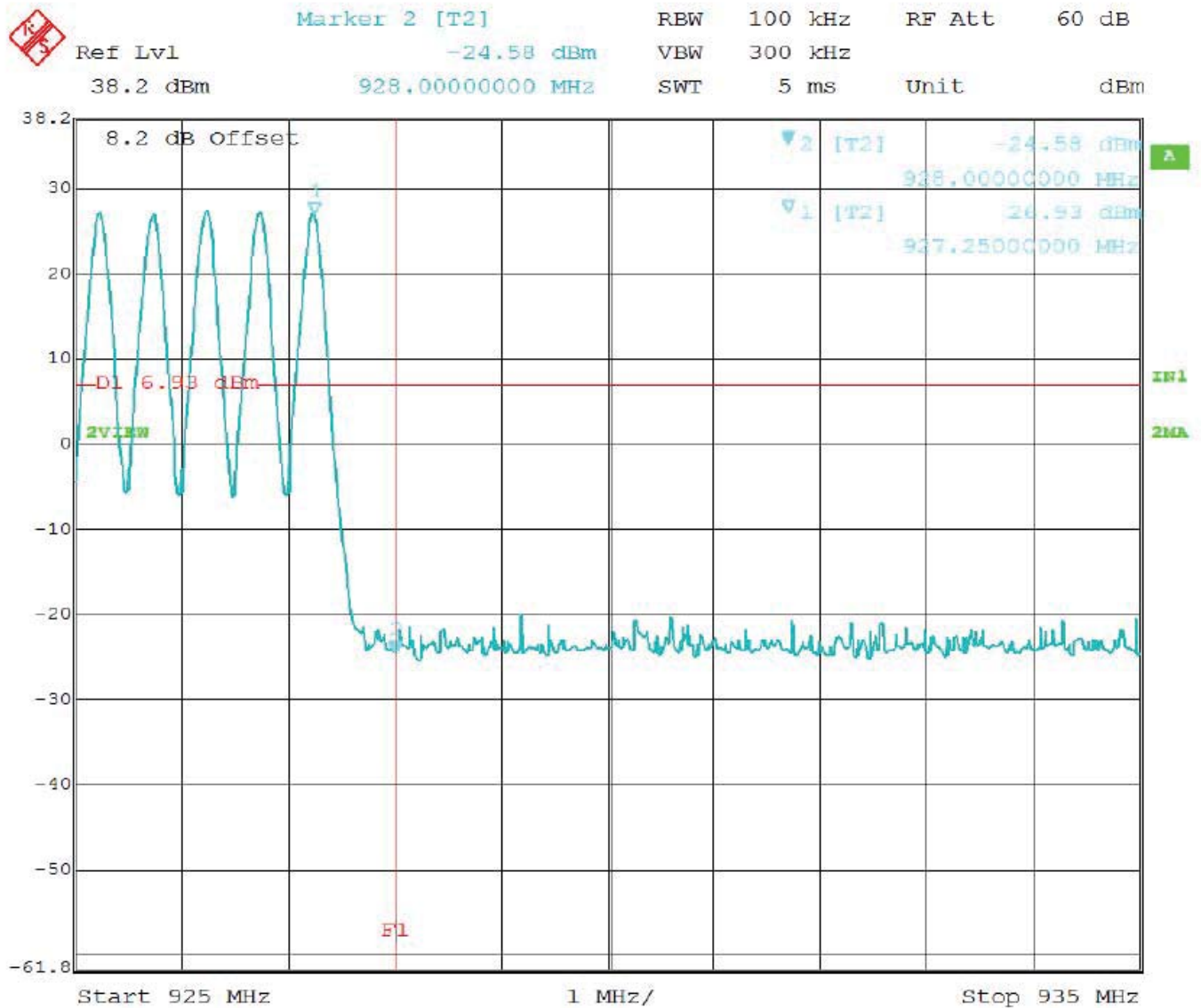
Band Edge – High Channel – Frequency Hopping Mode – Configuration #2 – Port #1 Worst Case
