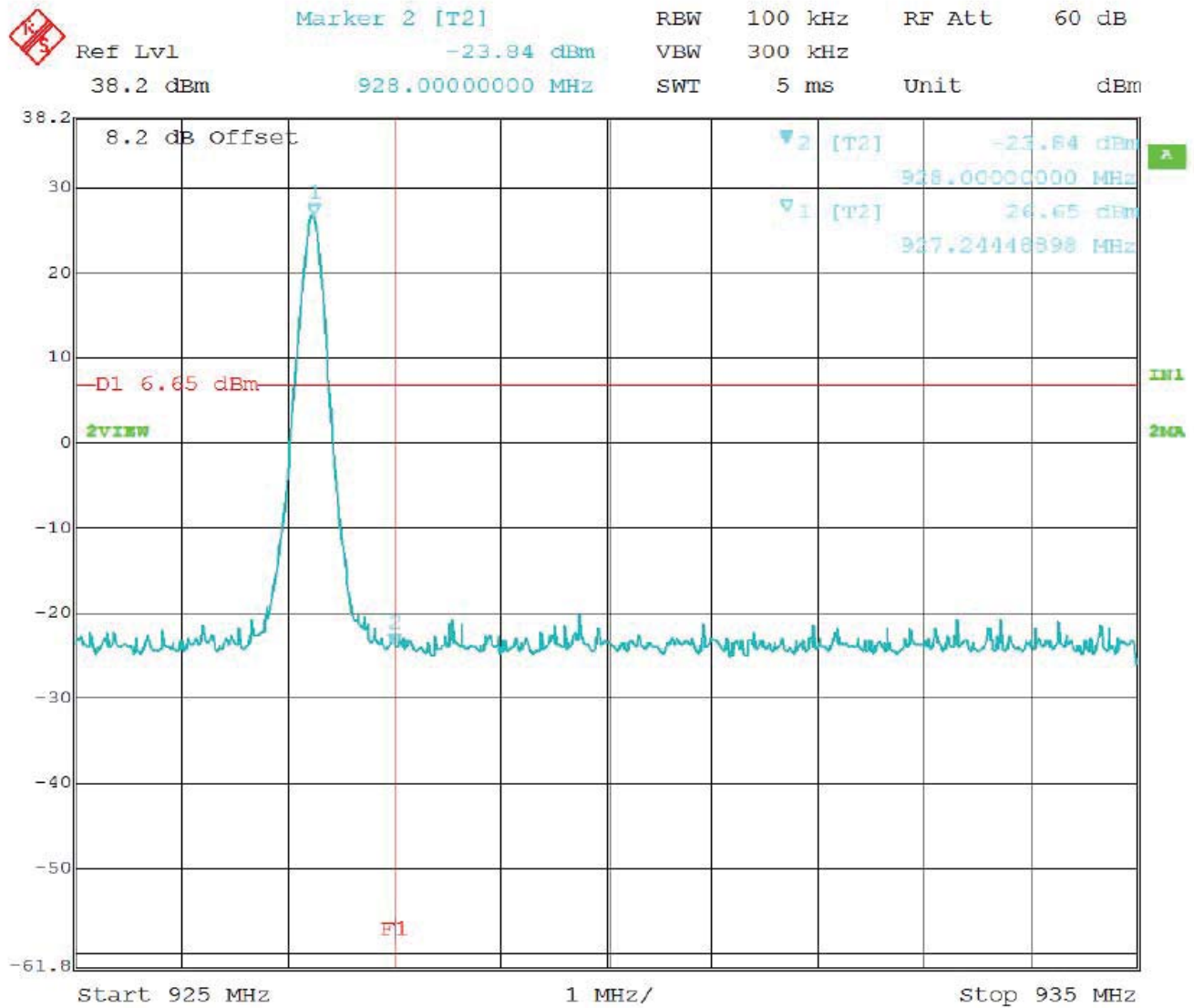
Band Edge – High Channel – Fixed Frequency Mode – Configuration #2 – Port #1 Worst Case
