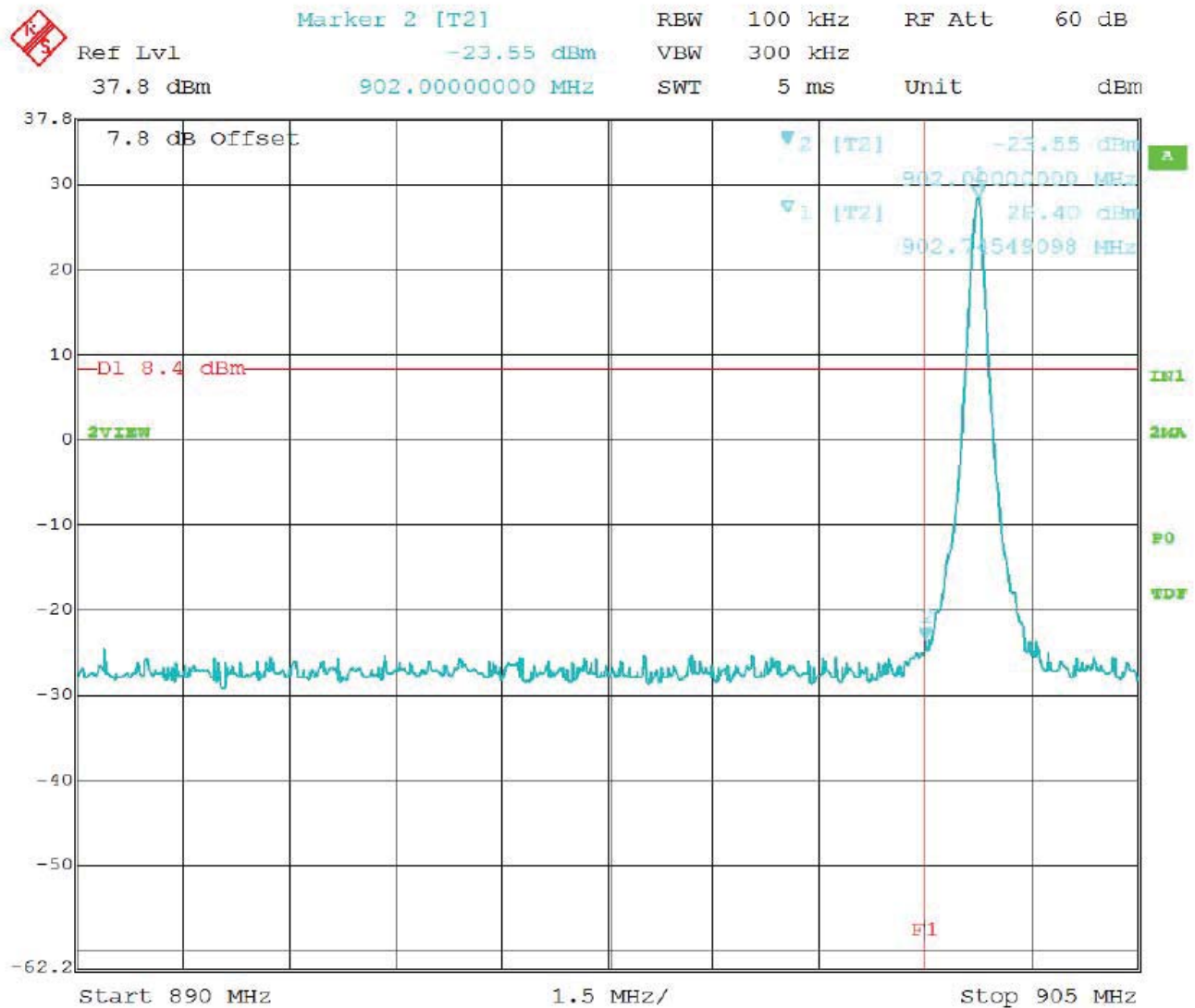
Band Edge – Low Channel – Fixed Frequency Mode – Configuration #1 – Port #4 Worst Case
