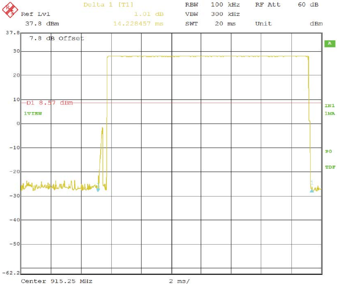
Time of One Pulse
