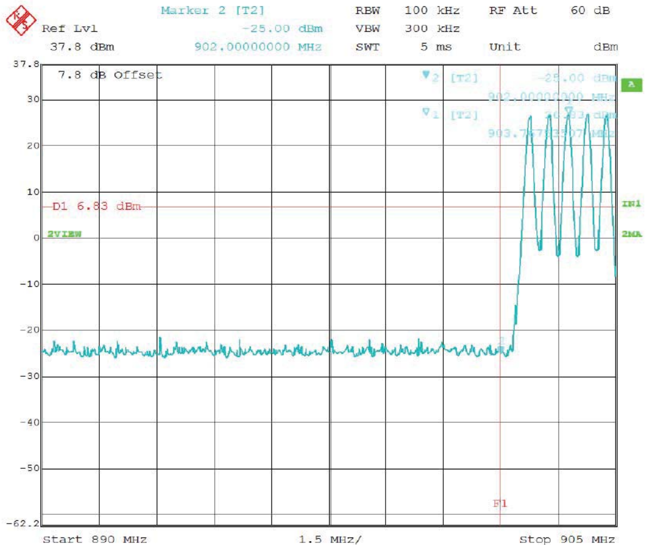
Band Edge – Low Channel – Frequency Hopping Mode – Configuration #2 – Port #1 Worst Case
