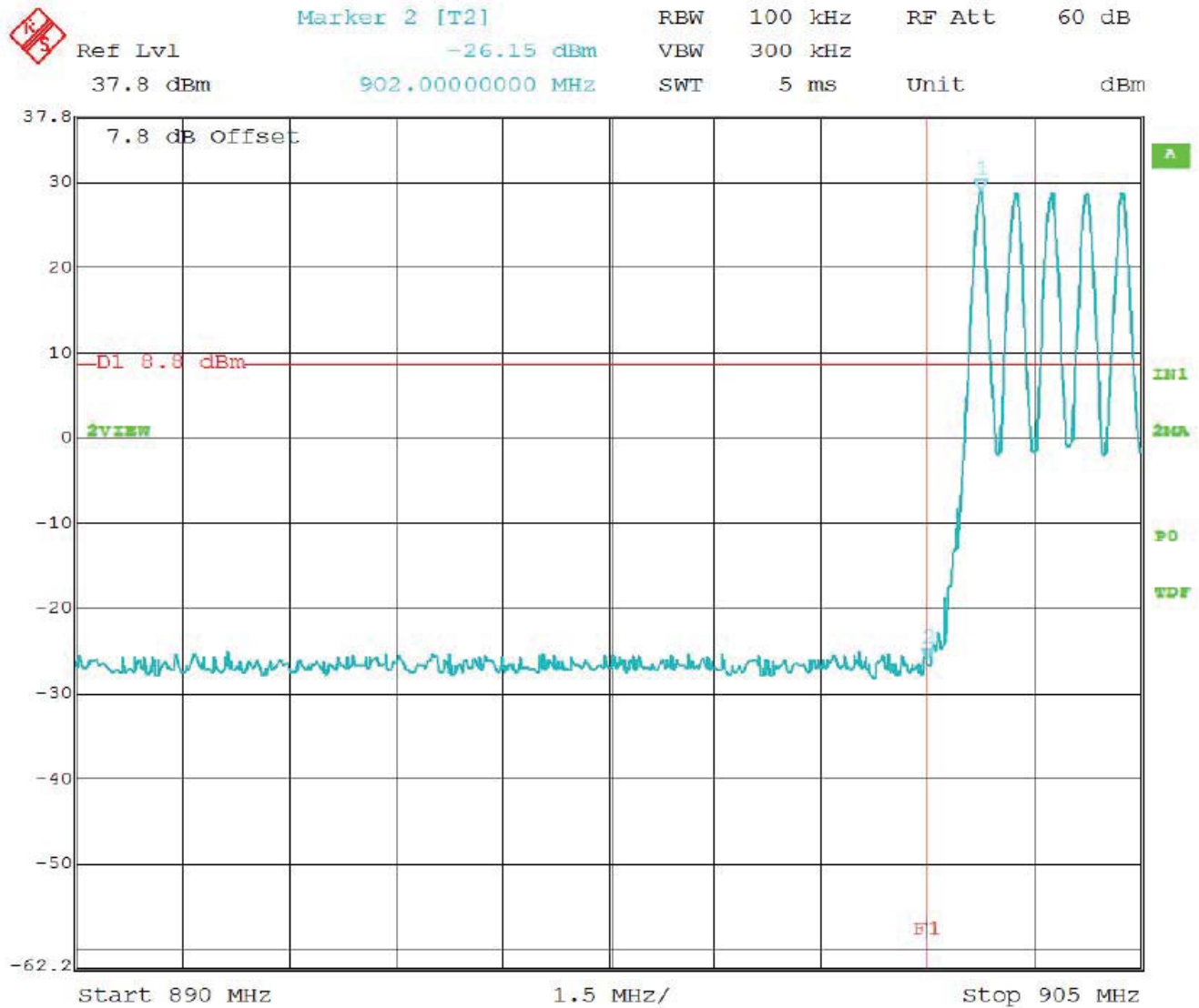
Band Edge – Low Channel – Frequency Hopping Mode – Configuration #1 – Port #4 Worst Case
