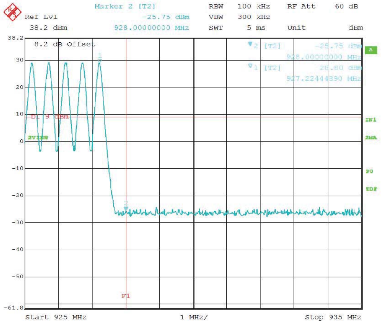
Band Edge – High Channel – Frequency Hopping Mode – Configuration #1 – Port #4 Worst Case
