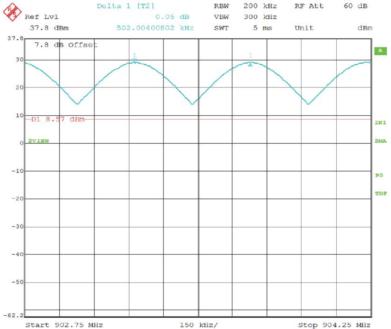
Channel Frequency Separation
