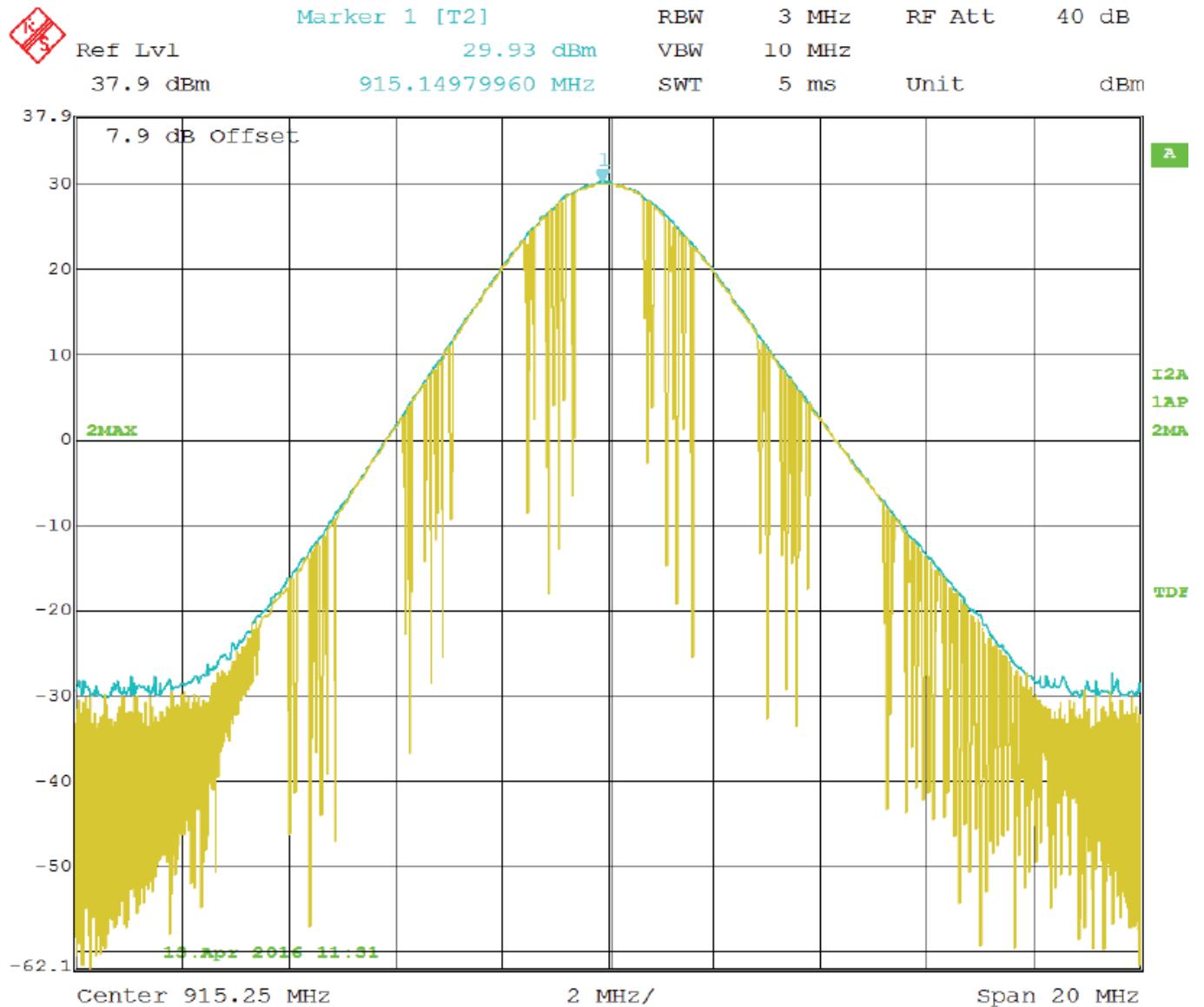
Peak Power Output – Middle Channel – Configuration #2 – Port #1 Worst Case
