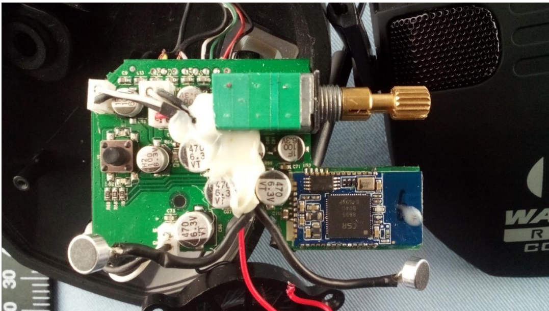
Main board component side
