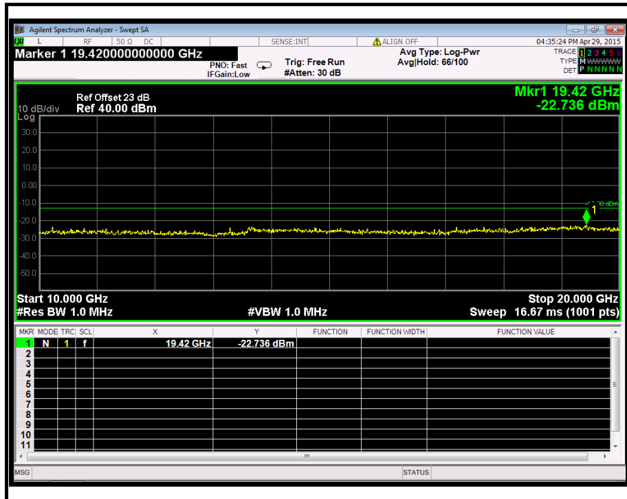
Figure 2-5: Out of Band emission at antenna terminals – HSDPA CH Mid
