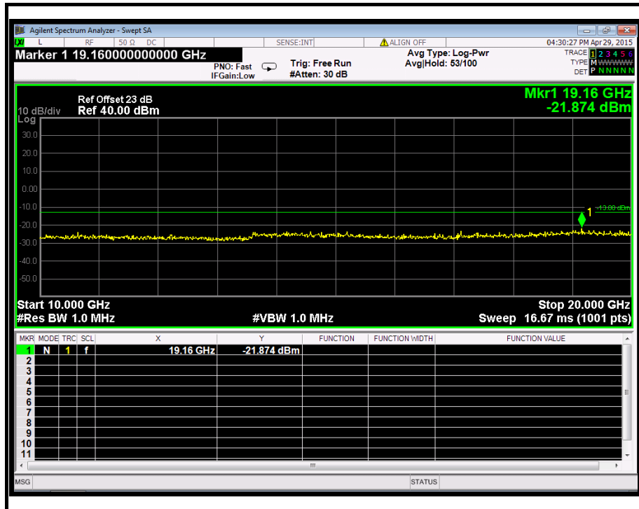
Figure 1-5: Out of Band emission at antenna terminals – HSDPA CH Low
