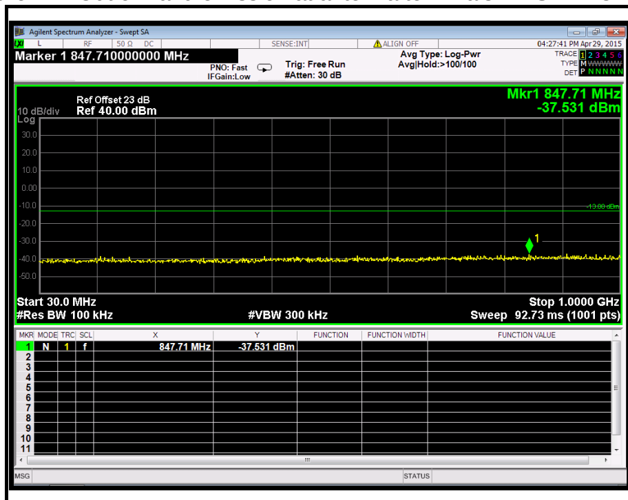
Figure 1-2: Out of Band emission at antenna terminals – HSDPA CH Low
