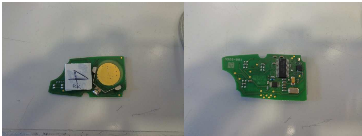
Figure 3.6-1: EUT overview
