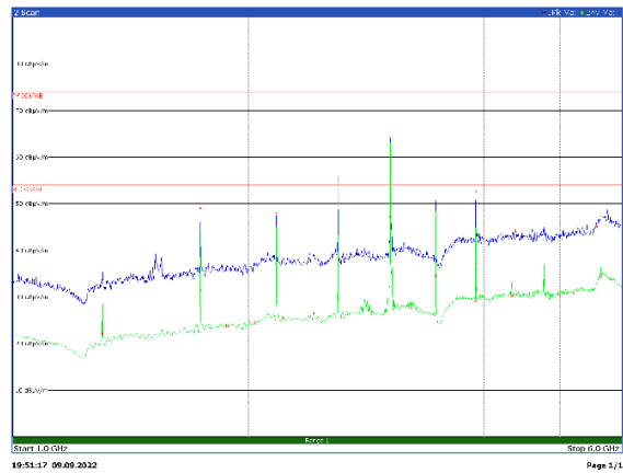
Figure 8.4-7: Horizontal polarization, Radiated spurious emissions above 1 GHz, E.U.T in vertical position
