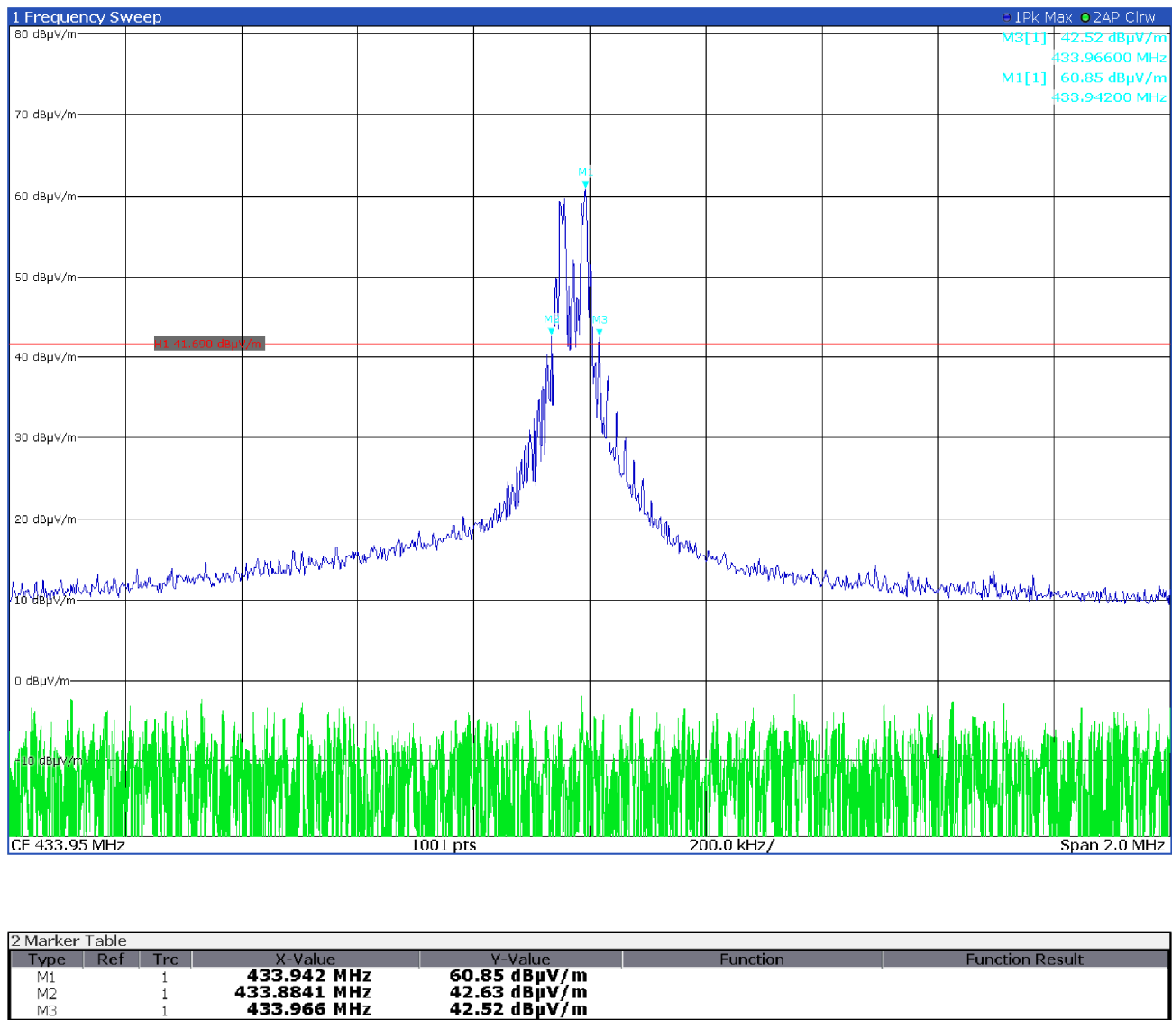
Figure 8.5-1: Occupied bandwidth measurement 20 dB = 433.966 MHz - 433.884 MHz = 0.082 MHz
