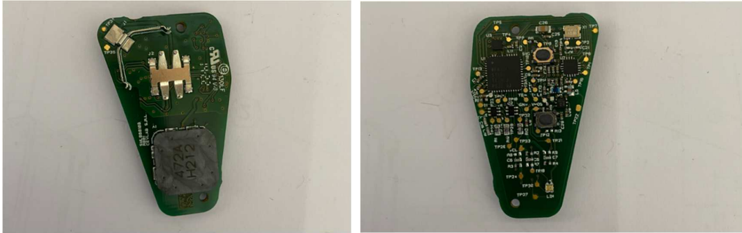
Figure 3.5-1: EUT overview
