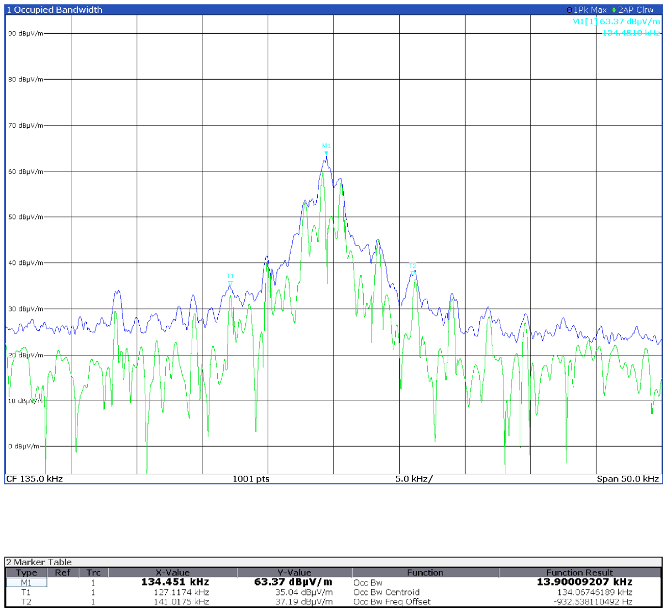
Figure 8.3-2: 99% Occupied bandwidth measurement = 13.9 kHz
