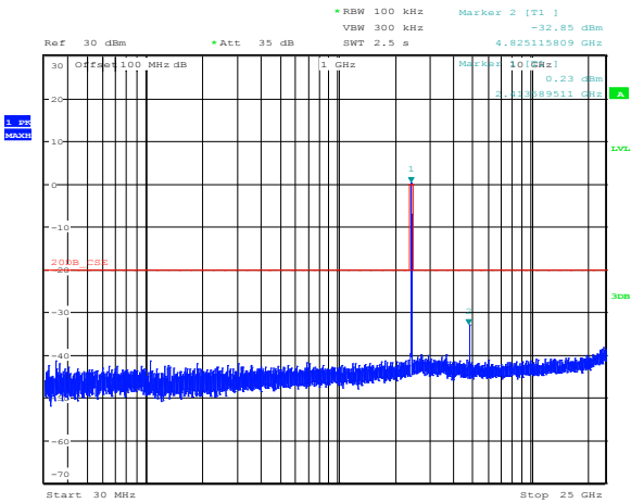
Figure 8.4-1: Conducted spurious emissions for 802.11b, low channel
