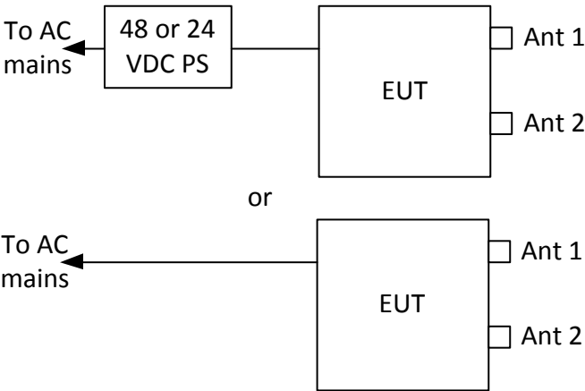
Figure 3.6-1: Setup diagram
