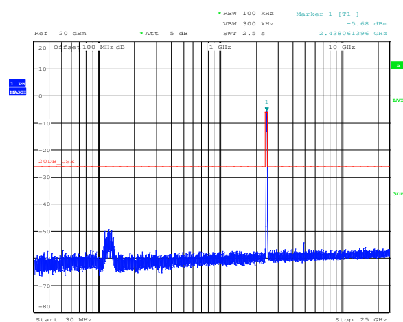
Figure 8.4-6: Conducted spurious emissions for 802.11g, mid channel
