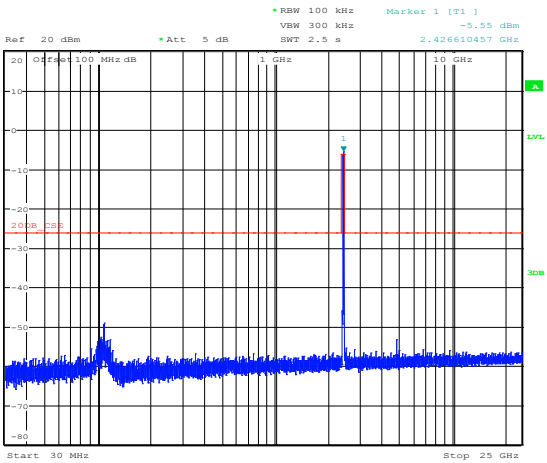
Figure 8.4-2: Conducted spurious emissions for 802.11g, low channel
