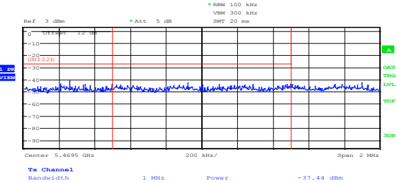
Figure 8.8-166: Lower band edge emission at 5470 MHz, channel 100, 802.11a, ch1
