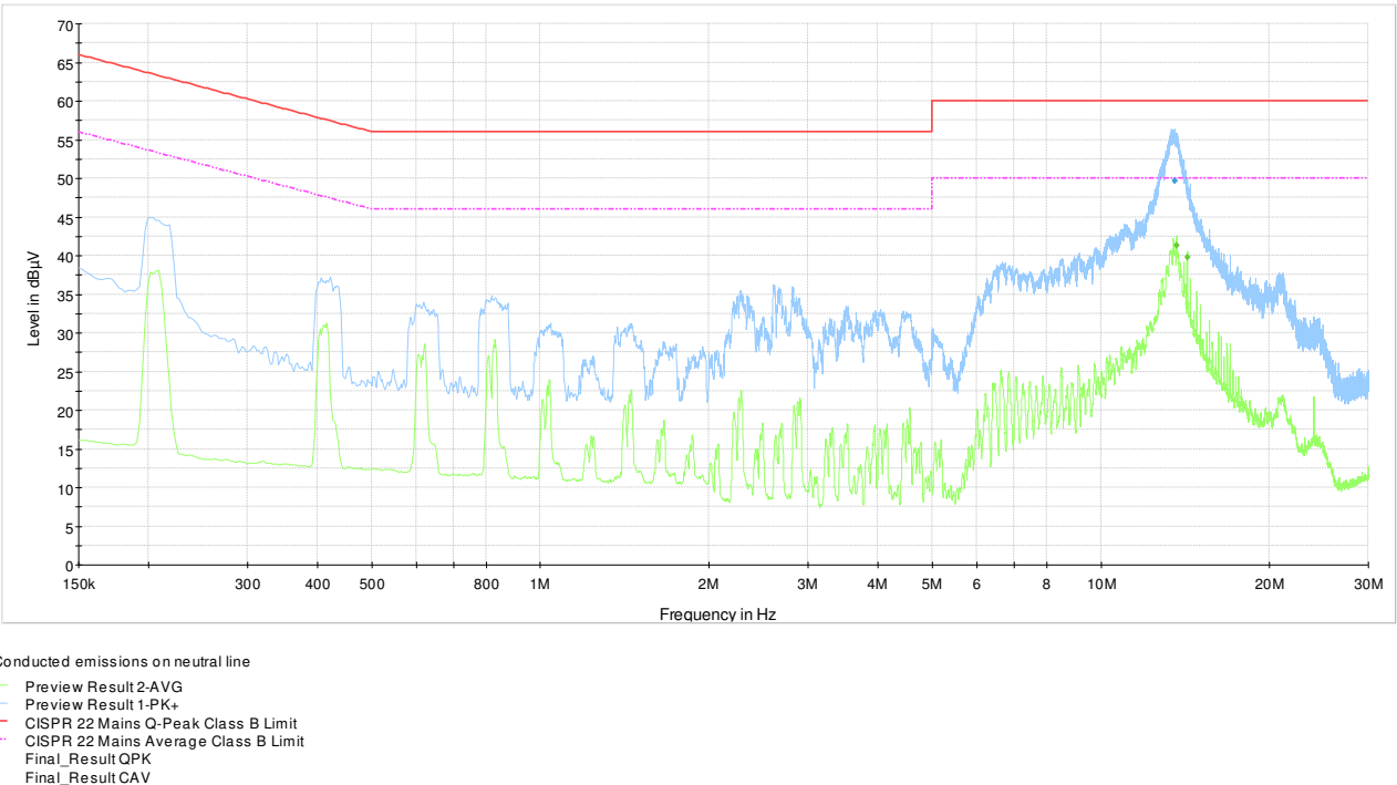
Plot 8.9-2: Conducted emissions on neutral line, 24 V DC PS
