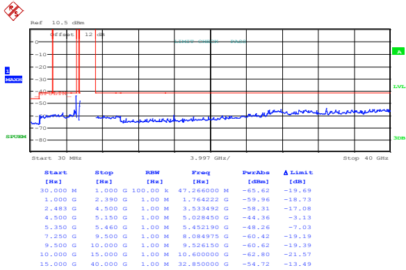
Figure 8.8-93: Spurious emissions within restricted bands at channel 54, 802.11n HT40, ch1
