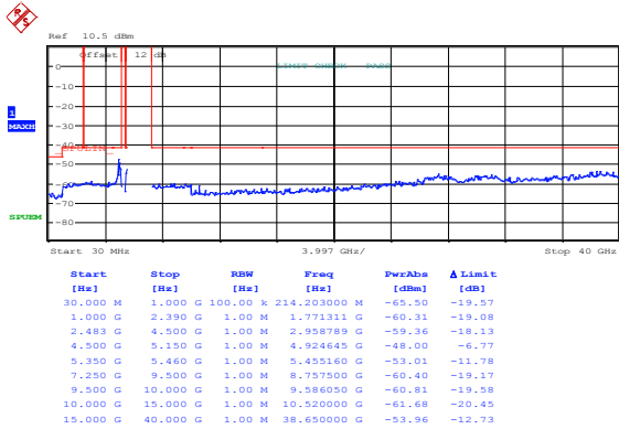
Figure 8.8-73: Spurious emissions within restricted bands at channel 48, 802.11a, cho
