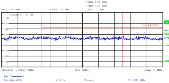
Figure 8.8-174: Upper band edge emission at 5850 MHz, channel 159, 802.11n HT40, ch1
