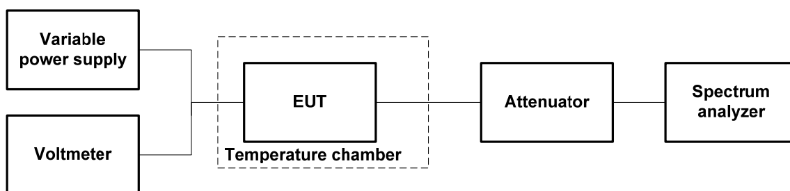
Photograph 7.6.1 Frequency stability test setup
