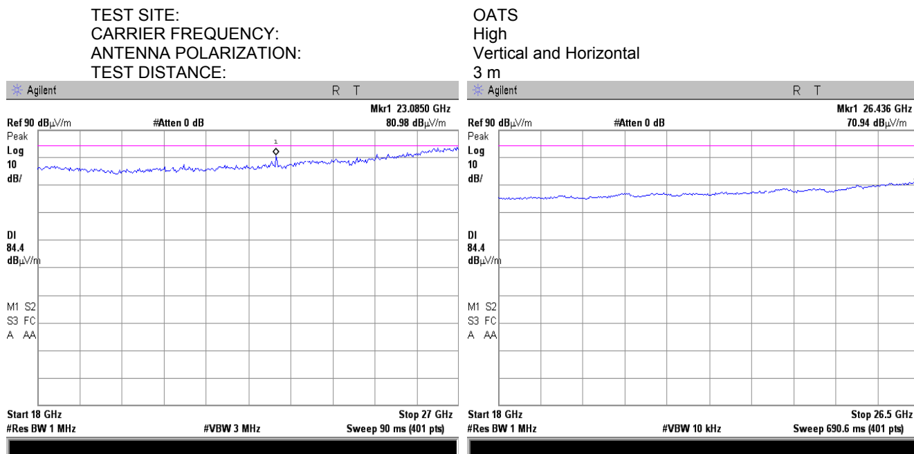
Plot 7.5.18 Radiated emission measurements in 18000 – 26900 MHz range
