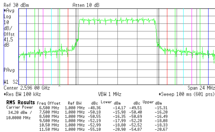
Plot 7.3.18 Spurious emission at band edges test results at high carrier frequency, 10 MHz EBW
