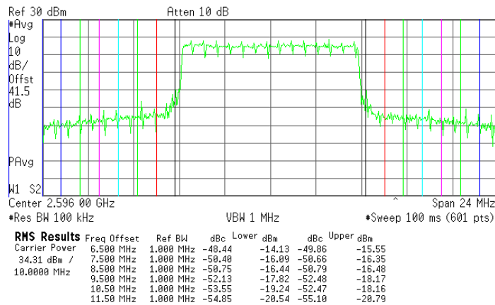
Plot 7.3.12 Spurious emission at band edges test results at high carrier frequency, 10 MHz EBW
