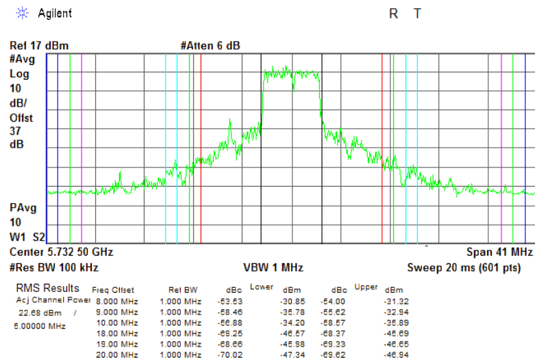
Plot 7.3.1 The highest band edge emission at low carrier frequency, 5 MHz BW, QPSK modulation, Antenna 1, 9.5 dBi gain
