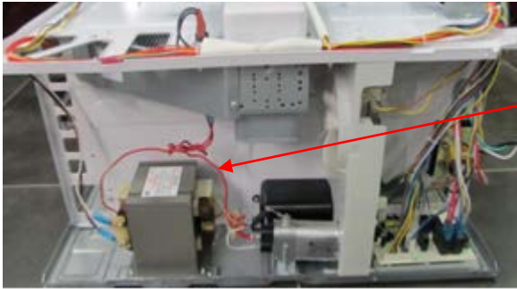
Original High-voltage transformer
