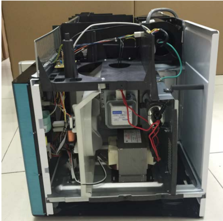
EUT Uncovered View
