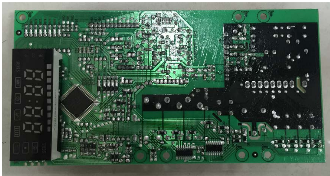
Mother board - Bottom View
