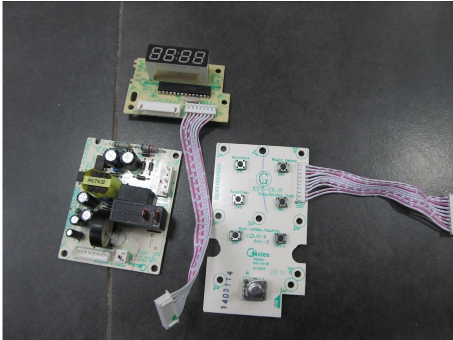
Mother board #1 - Top View(Touch pad)
