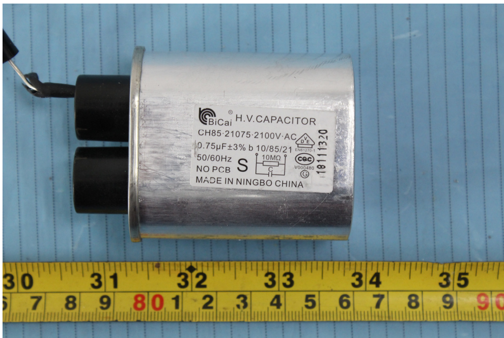
EUT – H.V. Capacitor View
