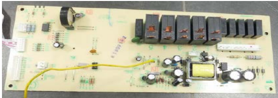
Original Mother board-top view
