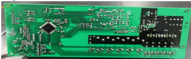
Original Mother board -bottom
