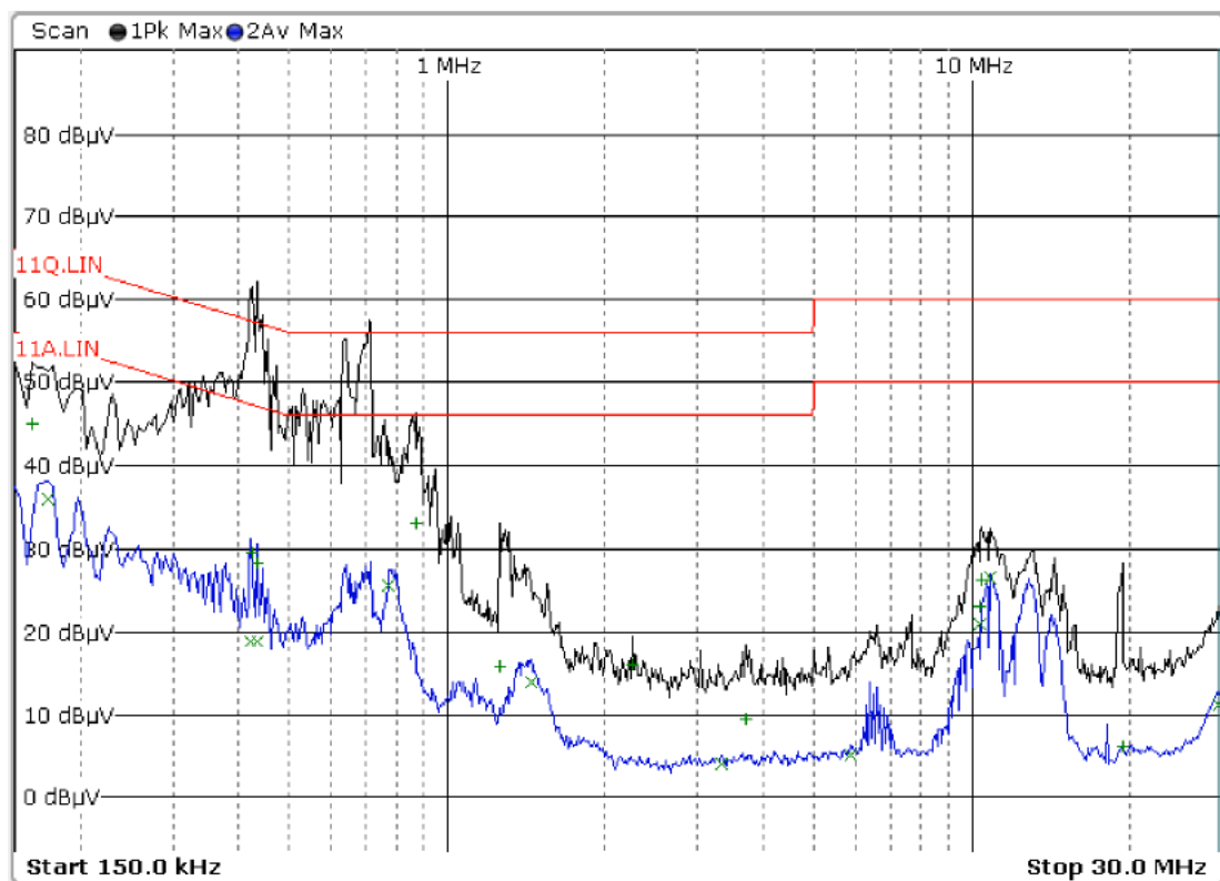
Line N Conducted Emission Graph
