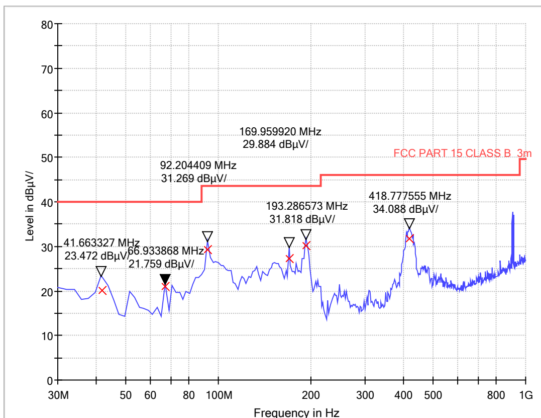
(Plot E: Test Antenna Horizontal 30M - 1G)
