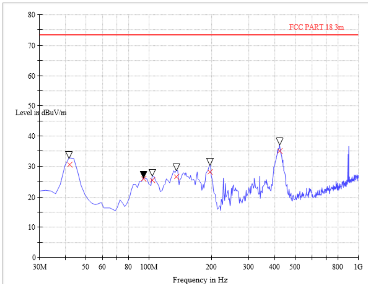
(Plot B: Test Antenna Vertical 30M - 1G)
