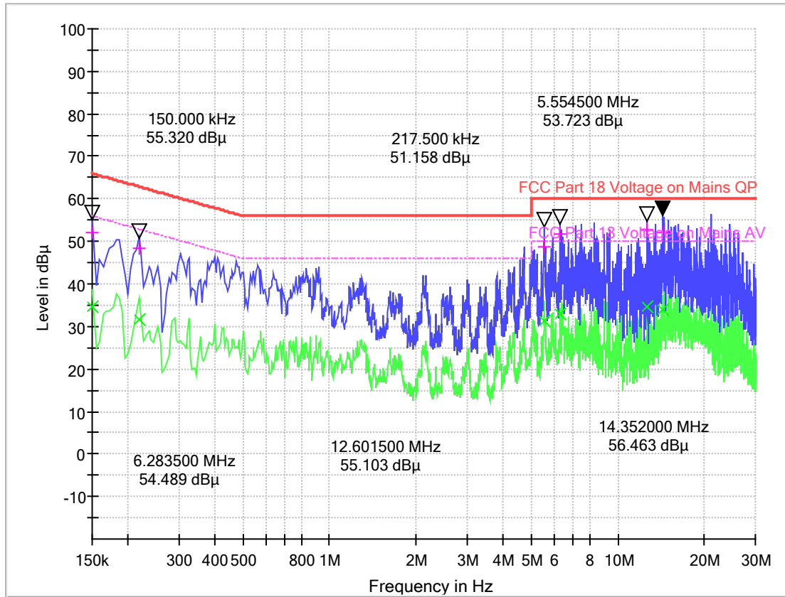
(Plot B: L2 Phase)
