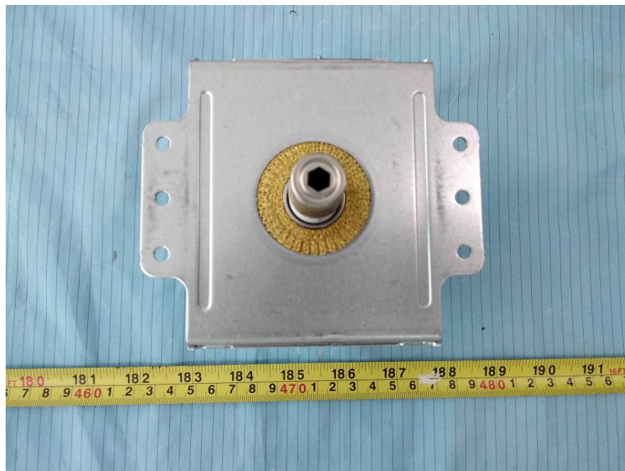
EUT – Magnetron Top View
