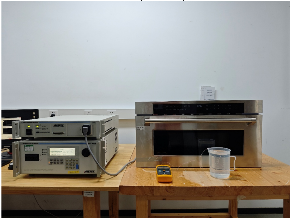
Power output test setup
