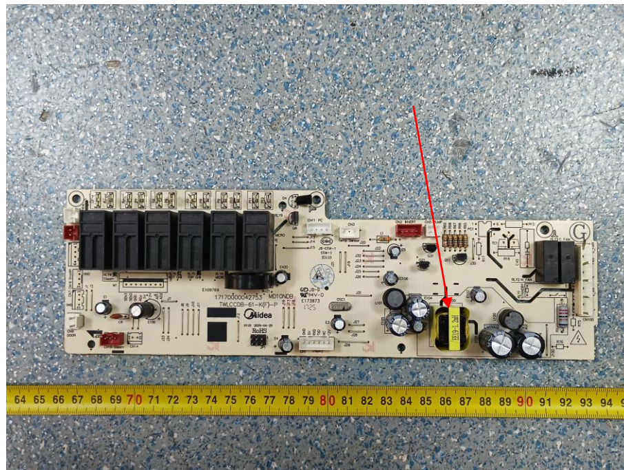
Transformer 1
