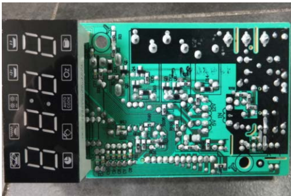
Mother board - Bottom View
