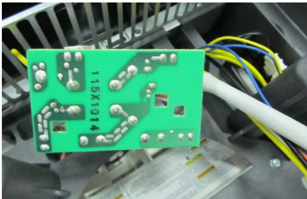
Power Filter Board Bottom View
