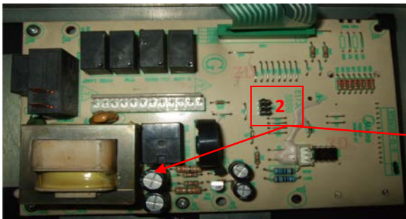
Original Mother board-top view
