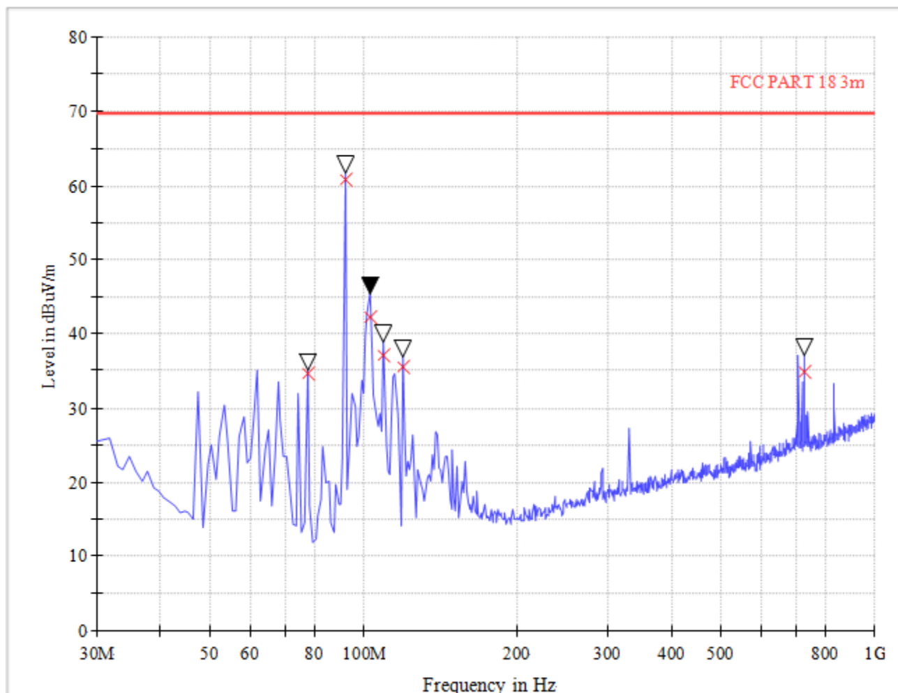
(Plot B: Test Antenna Vertical 30M - 1G)
