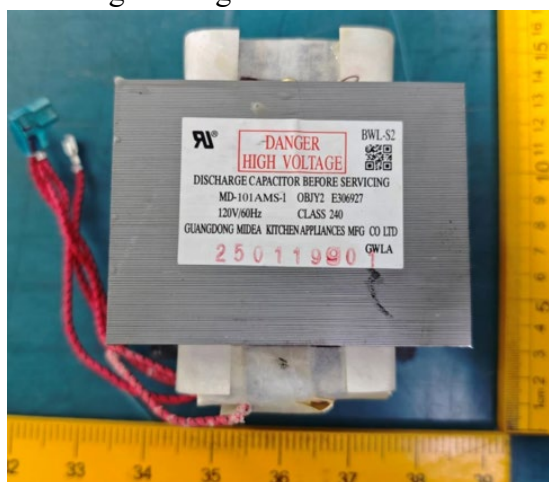
New high-voltage transformer
