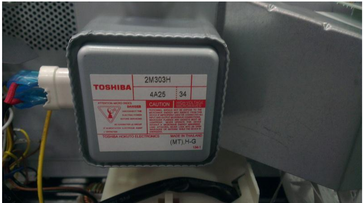
Magnetron Front View
