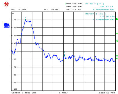
Port 2, 2483.5 MHz Band Edge
