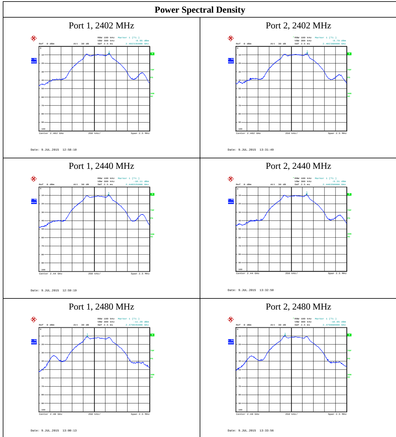
Plot 3. 1
