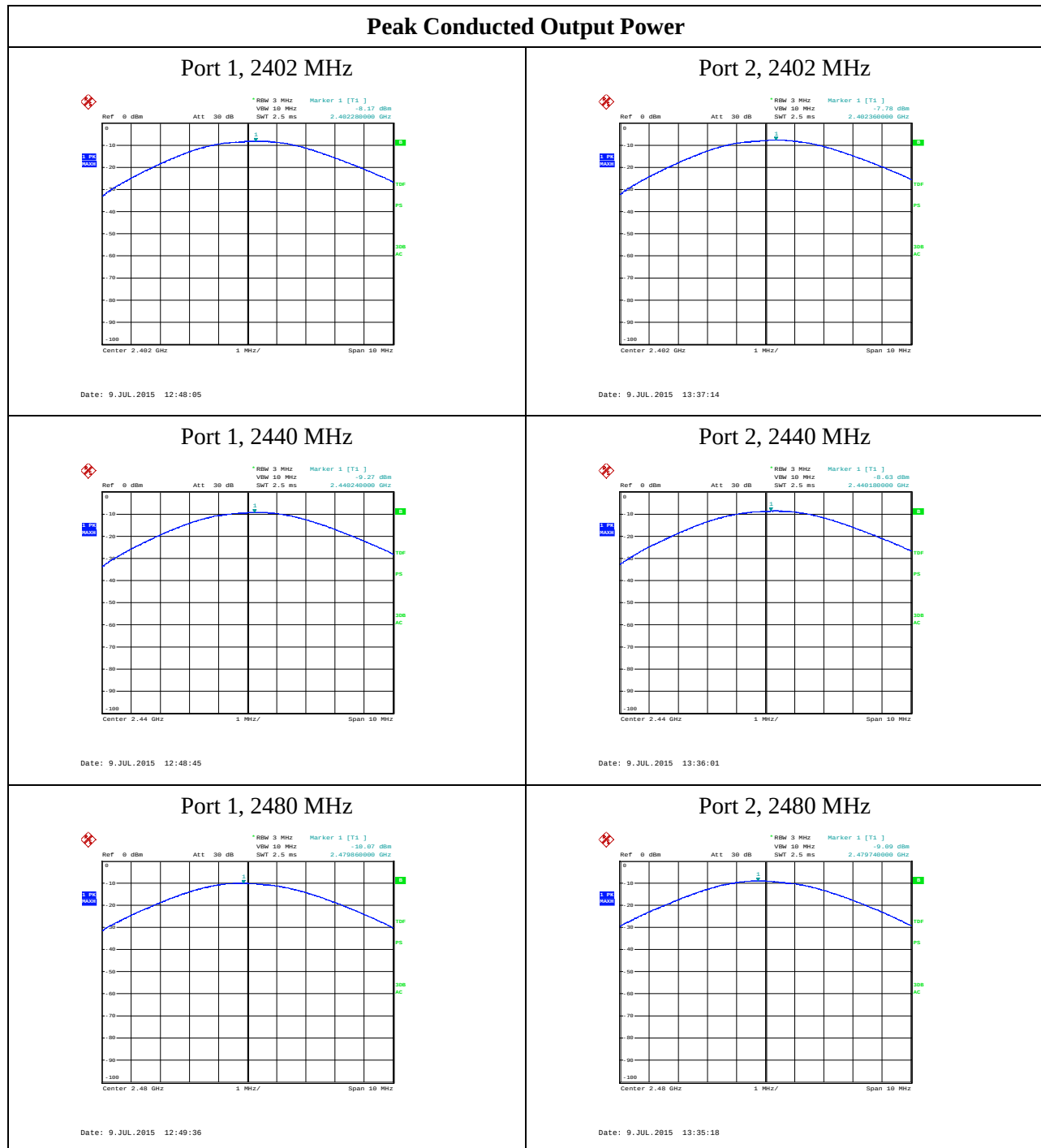
Plot 2. 1
